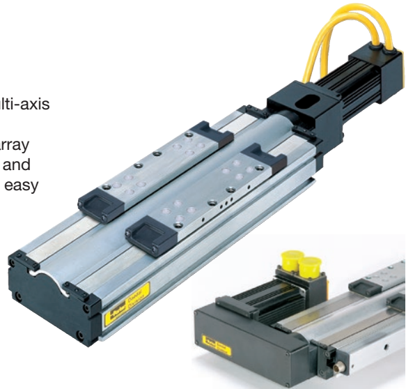
Parallel Motor Mount (with limit/home sensor pack option)
