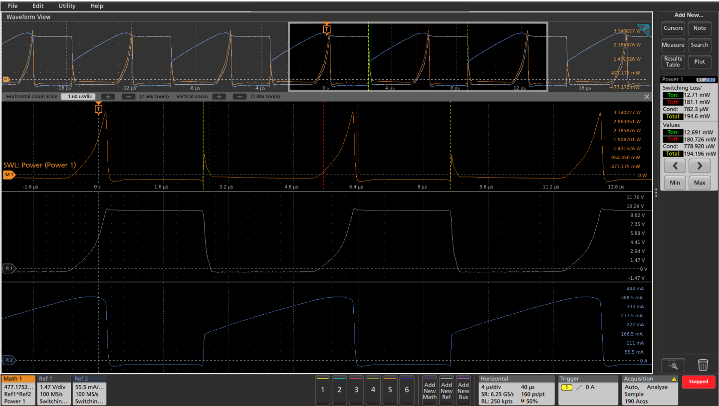
Switching Loss shows power dissipation in a FET. Waveforms are annotated with color-coded markers showing the measurement regions for T_{on} , T_{off} , and Total cycle, corresponding to values in the results badge. Controls in the results badge let you easily traverse from cycle to cycle.
