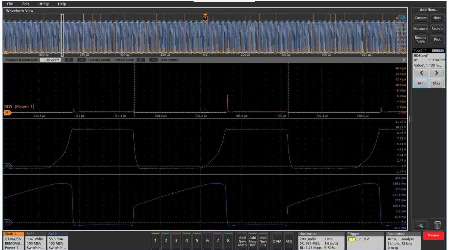
R_{DS(on)} measurement
