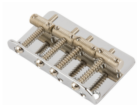
VINTAGE THREADED SADDLES Genuine Fender bass bridge assembly with nickel-plated steel bridge plate and four threaded barrel saddles.
