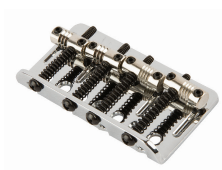
MODERN BASS BRIDGE Chrome plated steel bridge plate with partially threaded stainless steel saddles and string through body or top load option.
