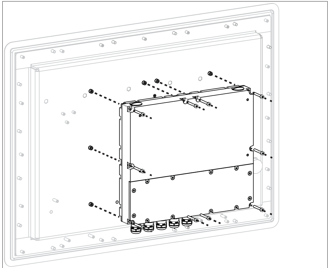
Figure 3.8 Mounting the TCU/PCU onto the display unit
