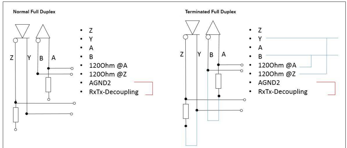
Figure 3.6 Full duplex cabling
