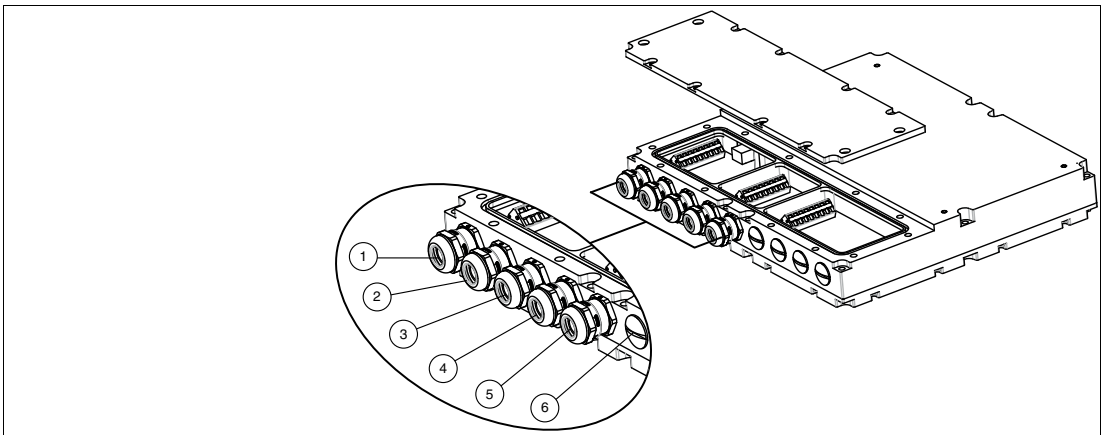
Figure 2.1 Cable gland connection layout
