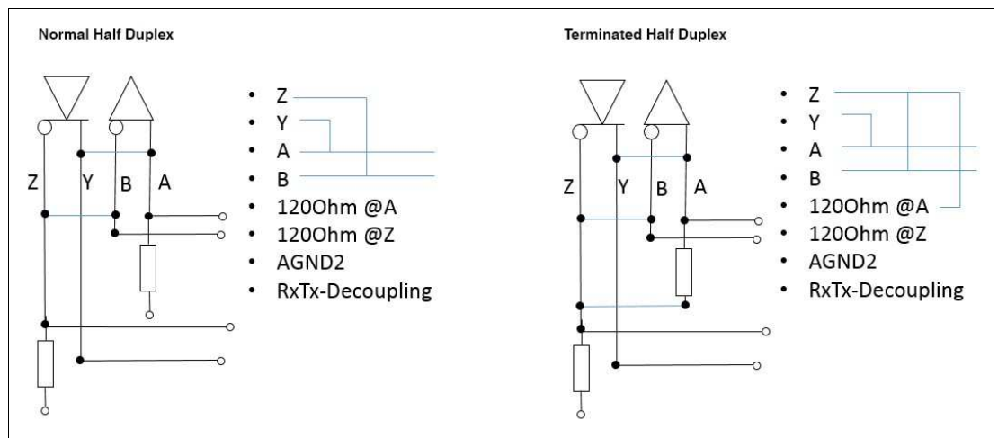
Figure 3.7 Half duplex cabling
