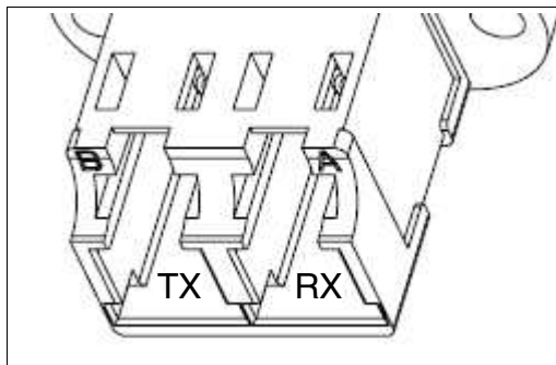
Figure 3.2 For the optional Fiber optic interface a duplex LC connection is required.
