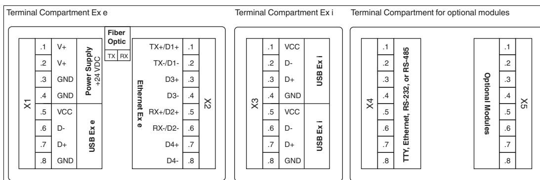
Figure 3.1 Terminal compartments
