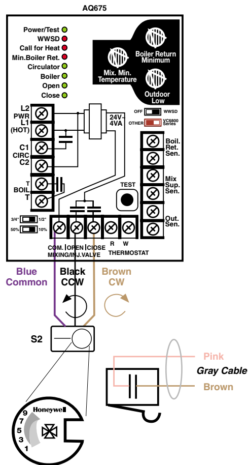
Fig. 6 M6063 wired to AQ675 Aquatrol Outdoor Temperature Compensator, right boiler water entry.
