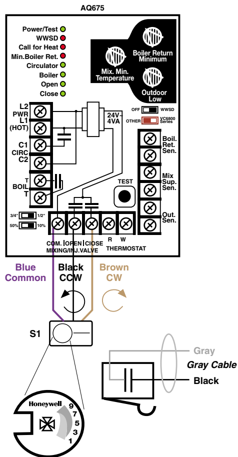
Fig. 5 M6063 wired to AQ675 Aquatrol Outdoor Temperature Compensator, left boiler water entry.
