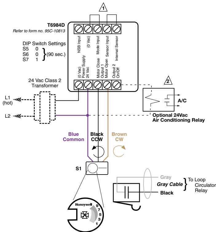
Fig. 7 M6063 wired to T6984D for room temperature control, boiler supply enters from left.
