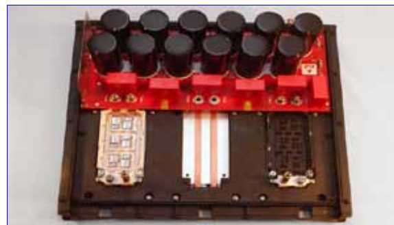
Figure 2: IGBT power semiconductor module (1200V 450A)
