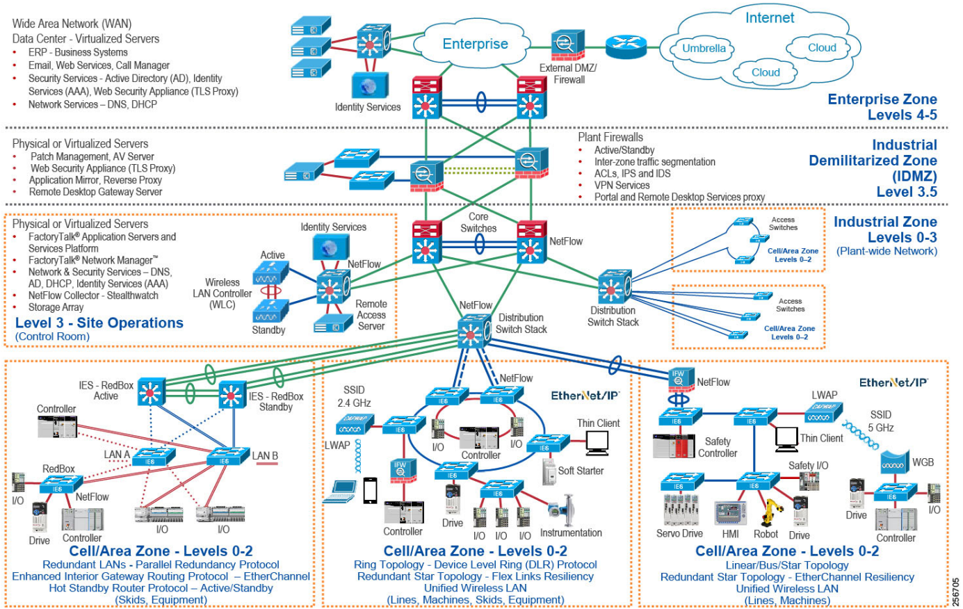
Figure 1-4 CPwE Architectures
