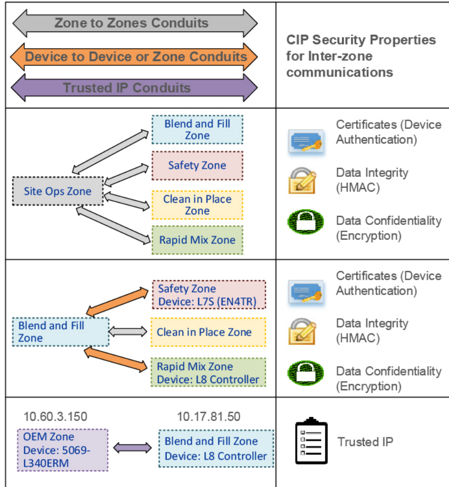
Figure 2-23 Inter-Zone Security
