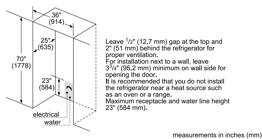
36" Freestanding Installation
