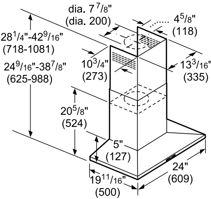
24" Pyramid Canopy Chimney Hood
