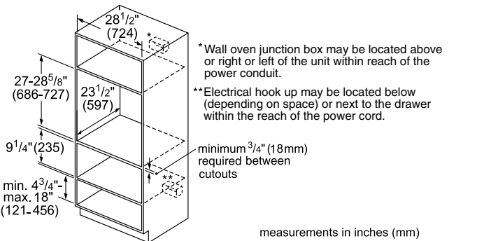
Standard Installation 30" Single Oven over Storage or Warming Drawer
