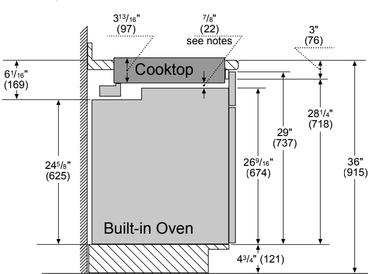
30" Cooktop Installation Above Wall Oven
