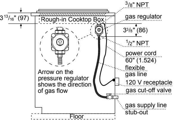
Gas Location
