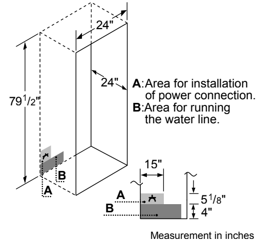
24" B11CB81SSS Installation
