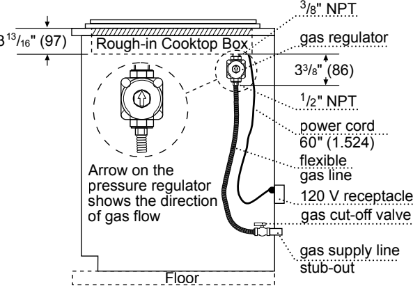
30" Cooktop Gas Location
