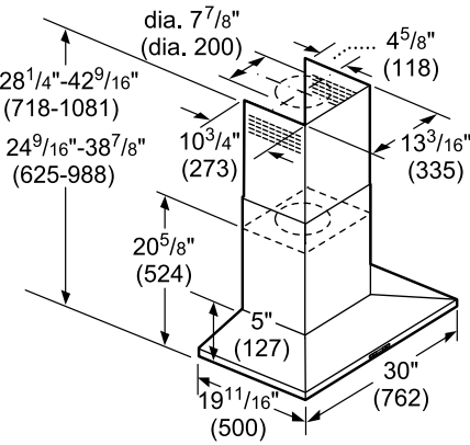
30" Pyramid Canopy Chimney Hood
