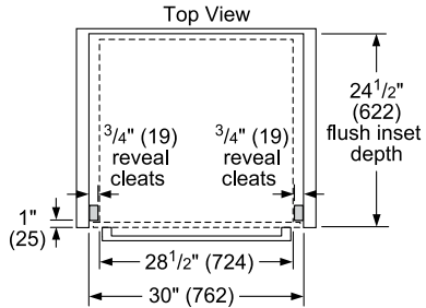
Flush Installation
