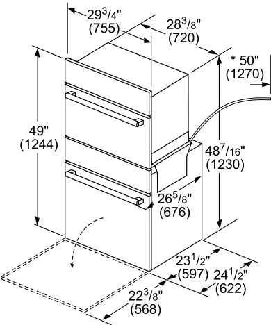
Product Dimensions
