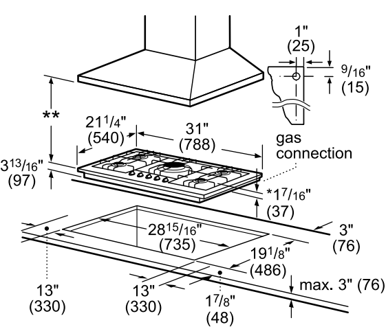
30" Cooktop and Cutout Dimensions
