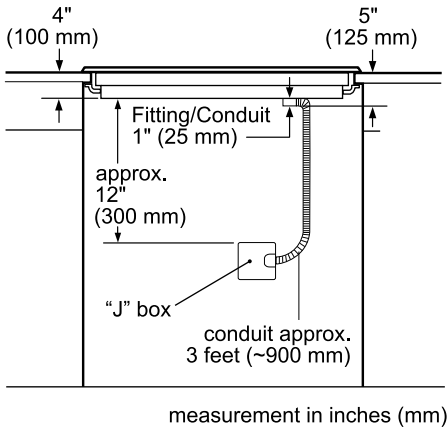
Gas Location
