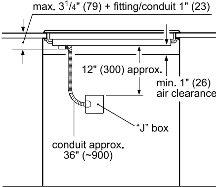
Electrical Location
