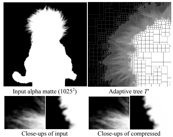
Figure 5: Compression of alpha matte (0.7 bpp; 51.2 dB)
