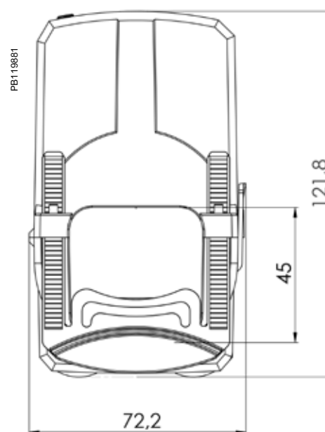
HP Dimensions
