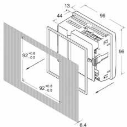
Dimensions PM5350IB
