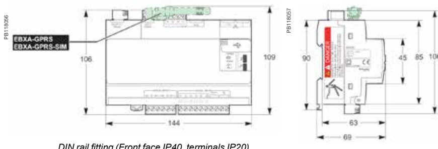
DIN rail fitting (Front face IP40, terminals IP20).
