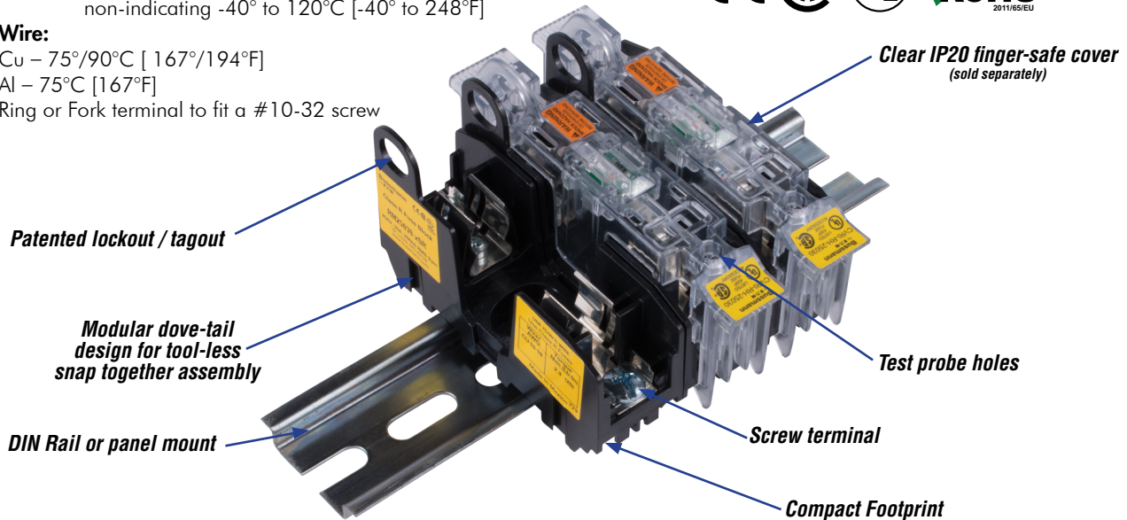
Modular Ferrule Fuse Blocks for Class R Fuses
