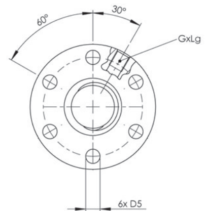
Hole pattern 3 NEFF standard
