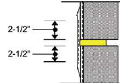
Fig. 3B Reinforce with mesh splice strip
