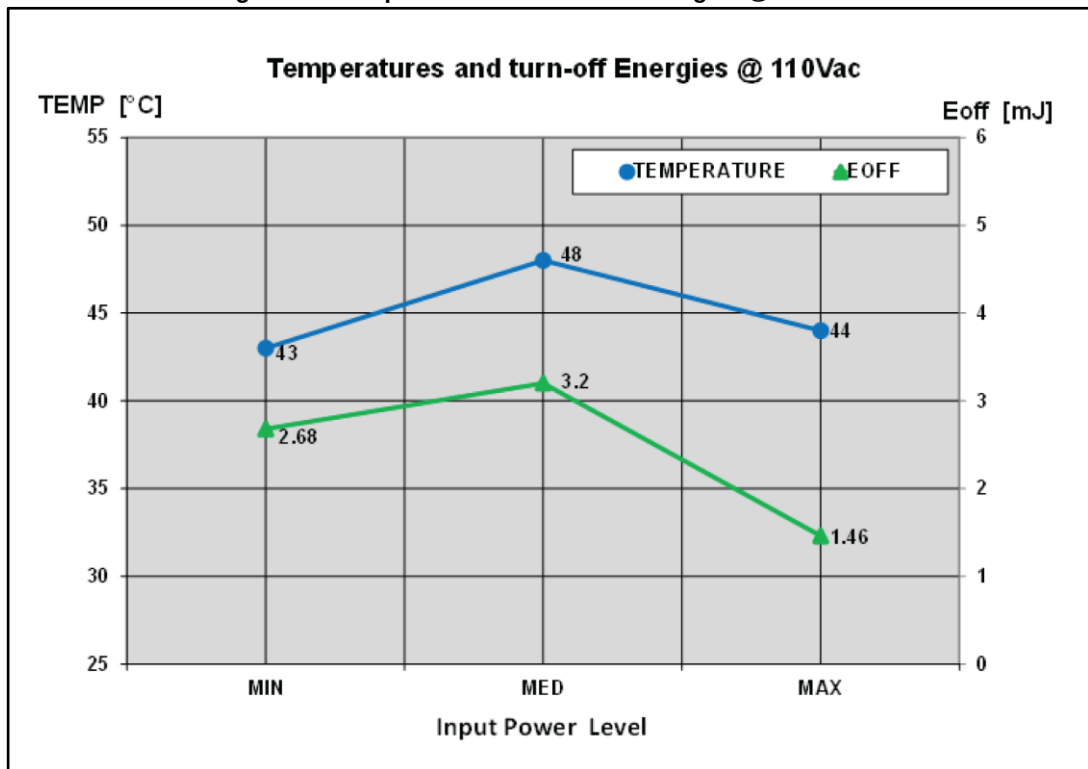
Figure 32: Temperatures and turn-off energies @ 110 VAC
