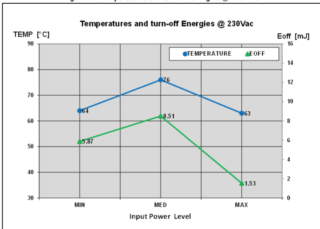
Figure 25: Temperatures and turn-off energies @ 230 VAC
