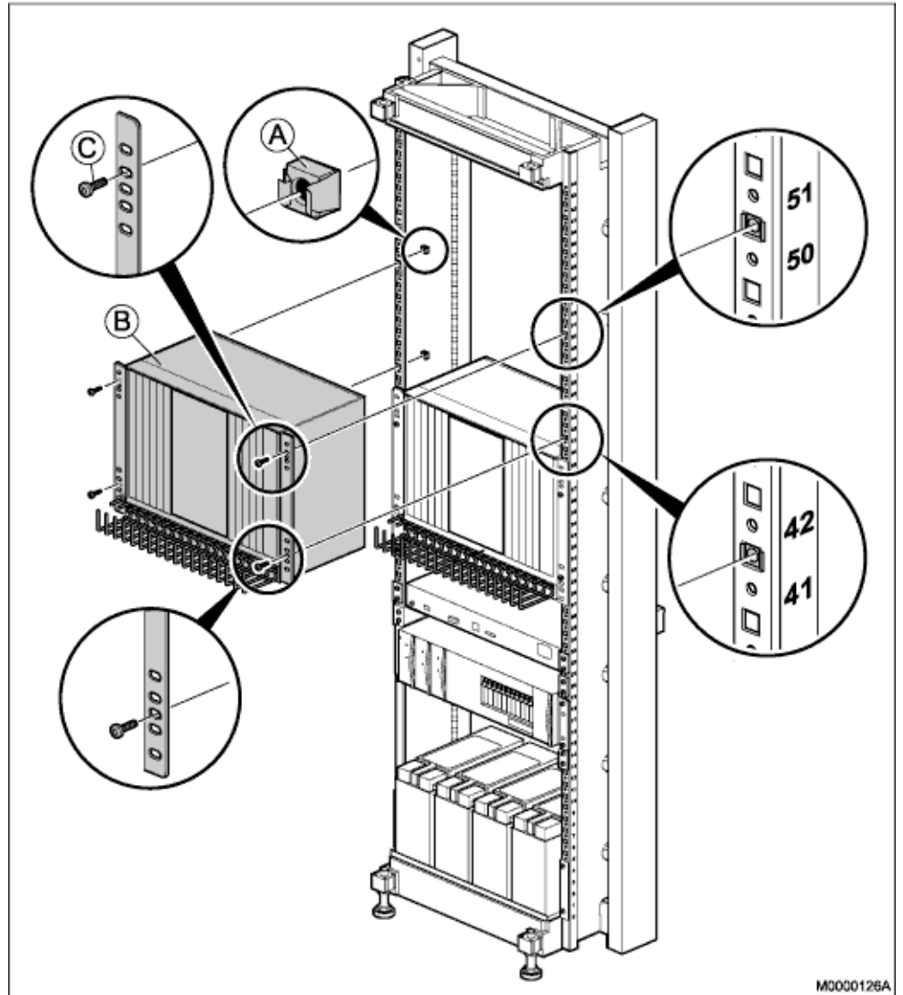
Figure 24: Installing Subrack A
