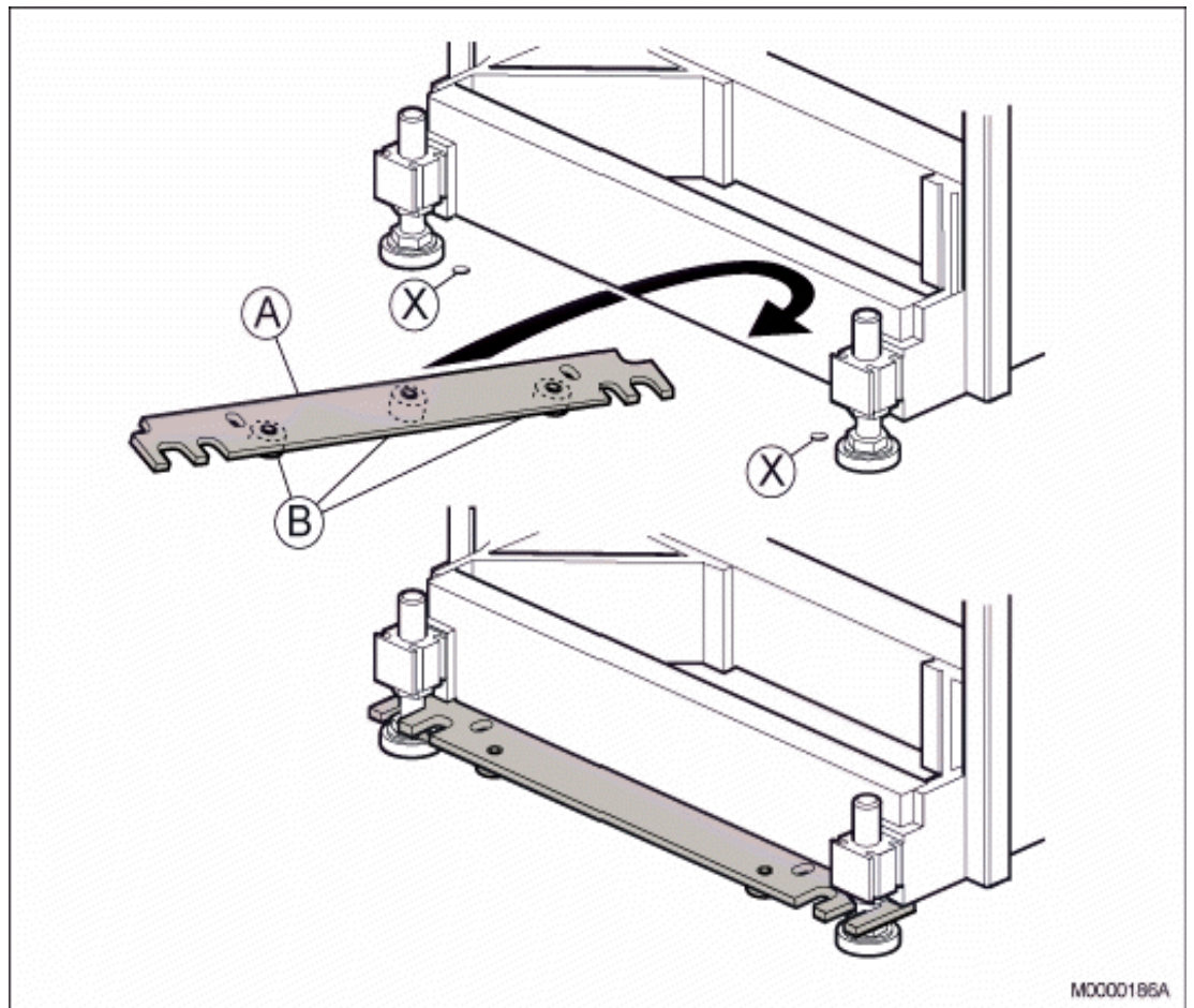
Figure 4: Installing the Tip Protection
