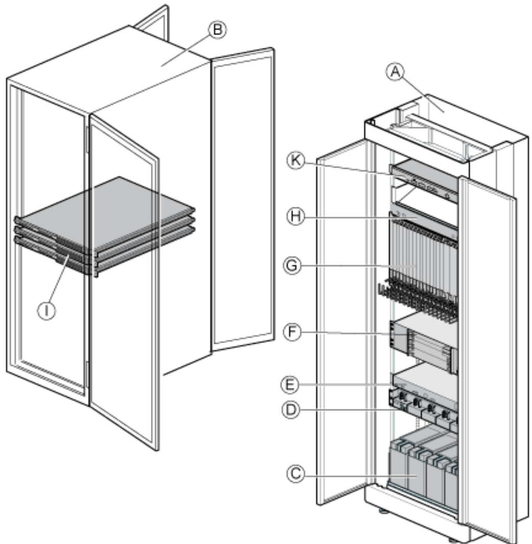
Figure 1: MX-ONE Cabinets
