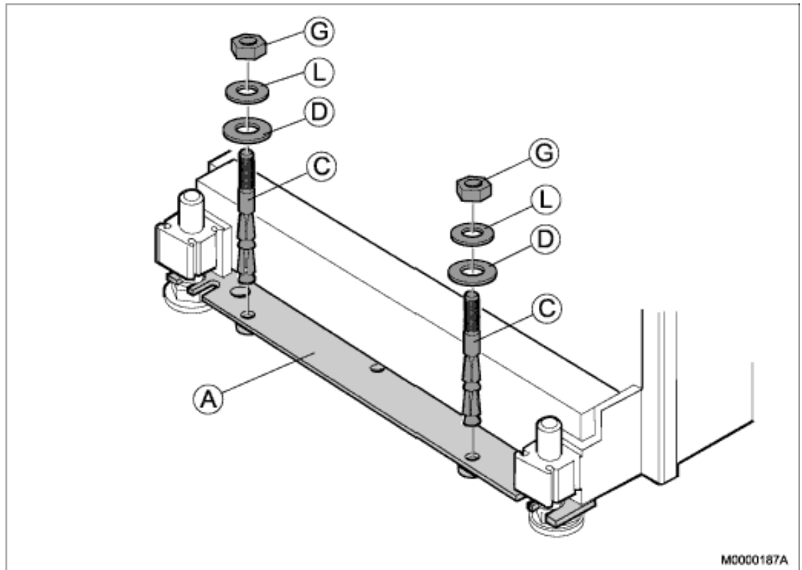
Figure 5: Installing the Expander Screw
