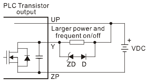
D: 1N4001 diode or equivalent component ZD: 9V Zener, 5W
