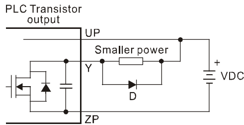
D: 1N4001 diode or equivalent component
