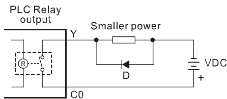
D: 1N4001 diode or equivalent component
