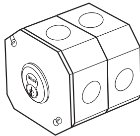
OC2 Deep octagon 3 1/2" x 3 1/2" x 3 1/4"
