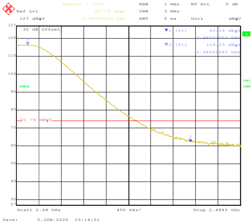
Figure 26: Band-edge-2480 MHz-H-Pk
