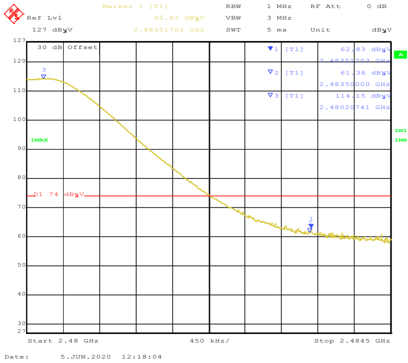
Figure 24: Band-edge-2480 MHz-V-Pk
