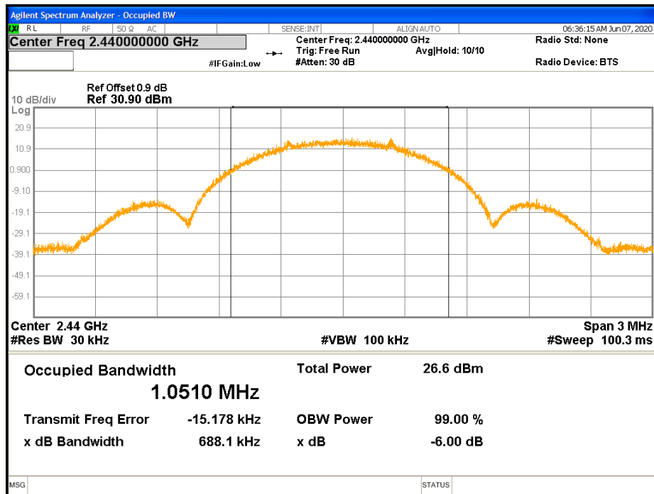
Figure 9: 99% Bandwidth-Transmitter -2440 MHz
