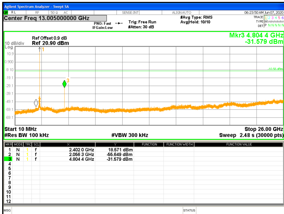
Figure 15: BLE Out of band Emission at 2402 MHz
