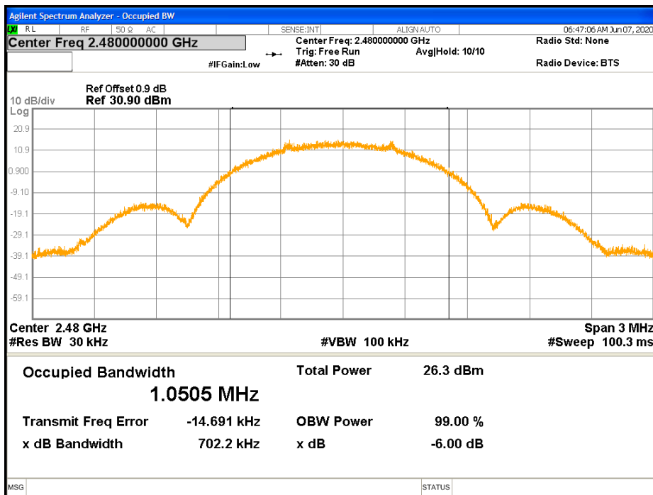
Figure 10: 99% Bandwidth-Transmitter -2480 MHz
