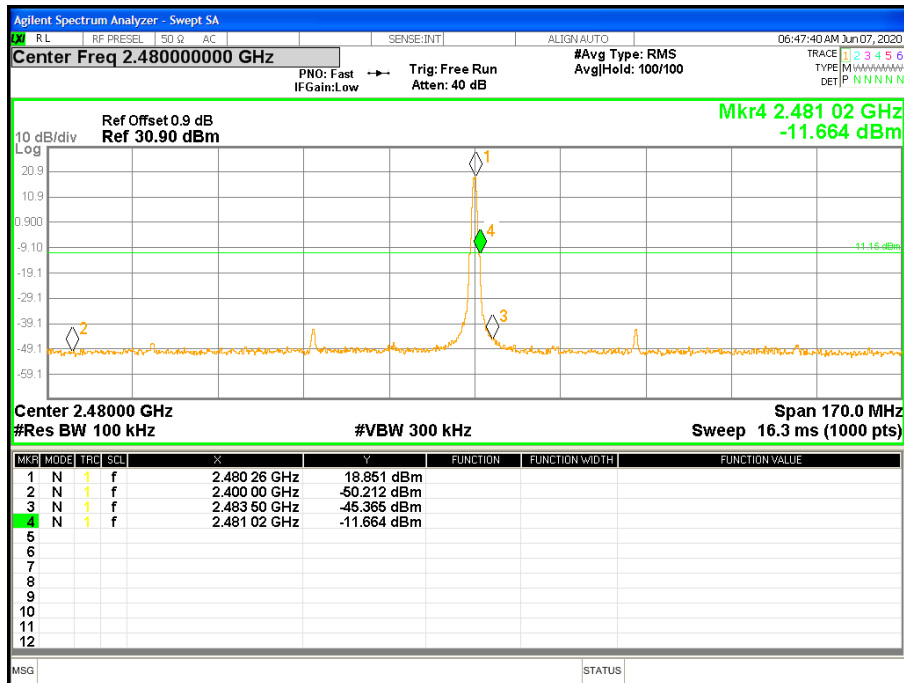
Figure 18: BLE Conducted Band Edge at 2480 MHz
