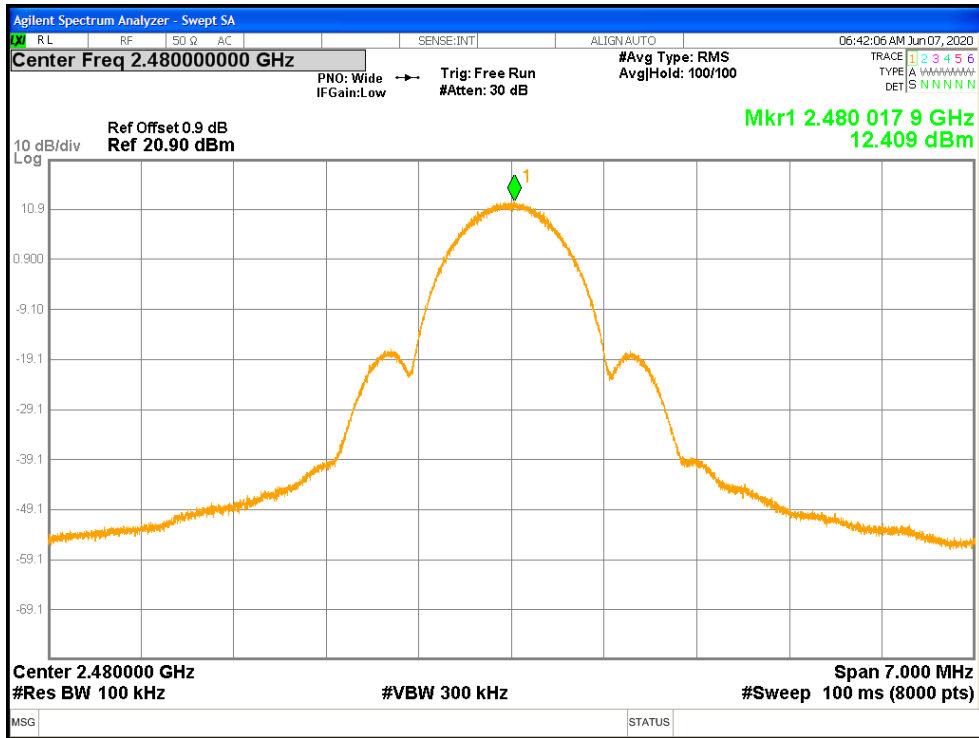
Figure 13: BLE Maximum Power Spectral Density-2480 MHz
