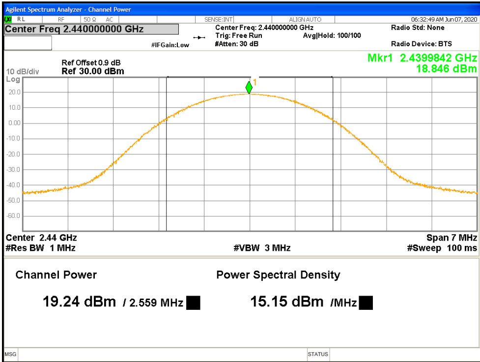
Figure 3: BLE Maximum Conducted Output Power at 2440 MHz
