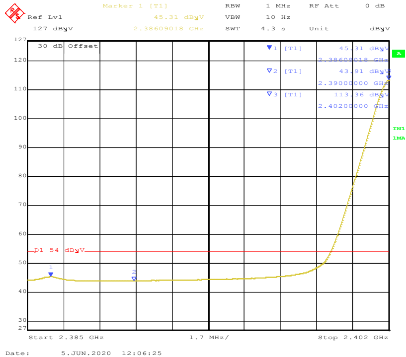
Figure 23: Band-edge-2402 MHz-H-Avg
