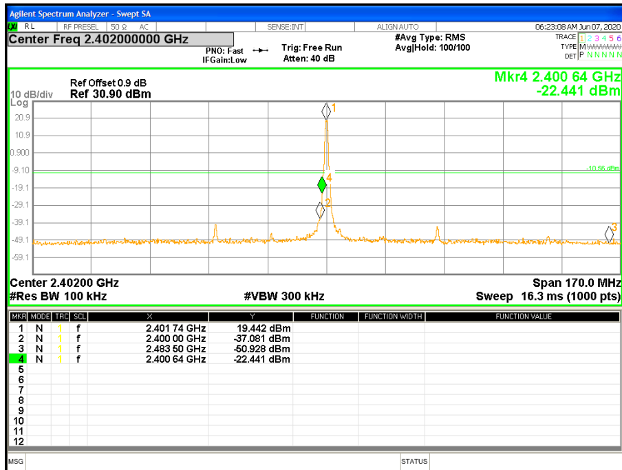
Figure 14: BLE Conducted Band Edge at 2402 MHz
