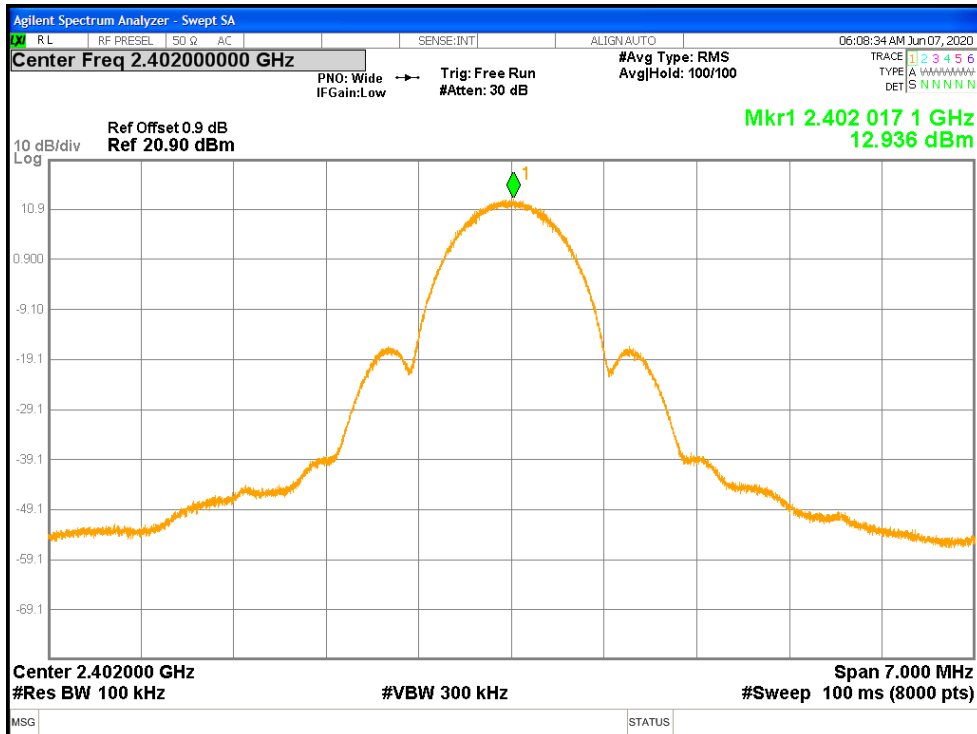
Figure 11: BLE Maximum Power Spectral Density-2402 MHz
