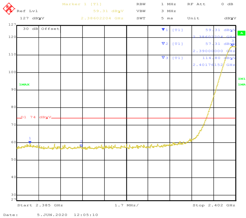
Figure 22: Band-edge-2402 MHz-H-Pk
