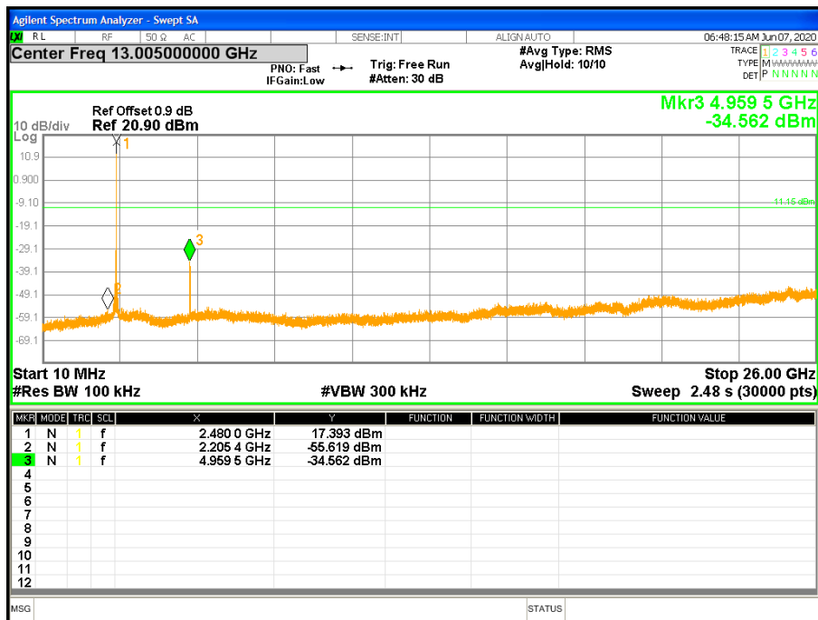
Figure 19: BLE Out of band Emission at 2480 MHz
