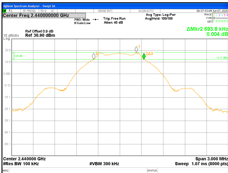
Figure 6: DTS Bandwidth-Transmitter -2440 MHz
