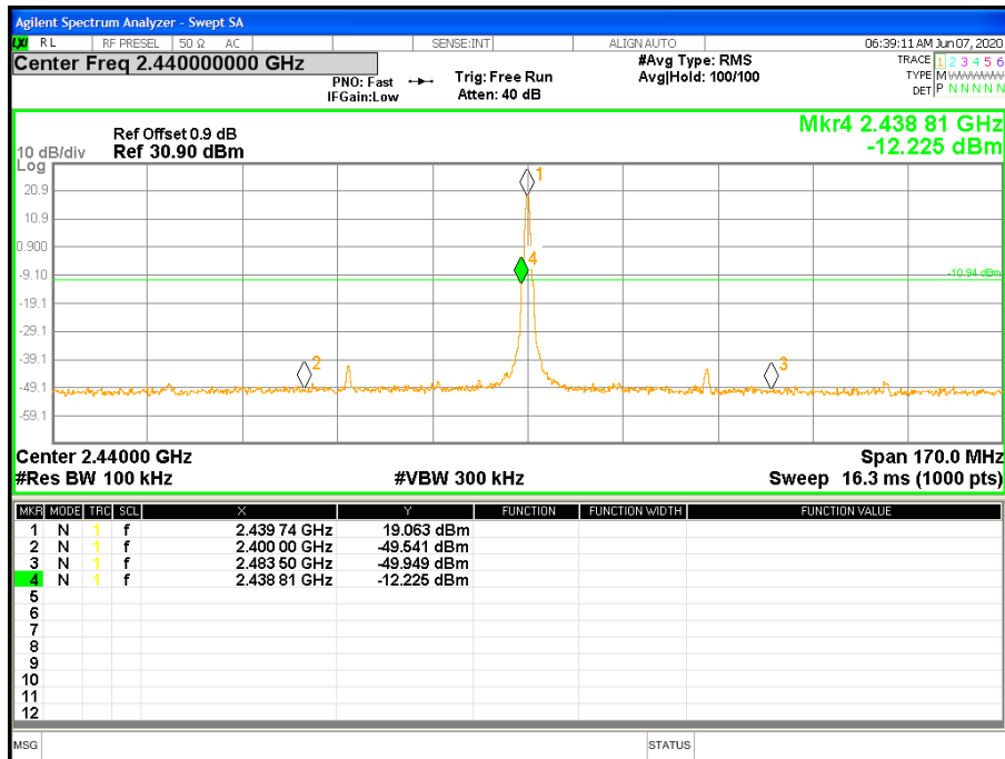
Figure 16: BLE Conducted Band Edge at 2440 MHz
