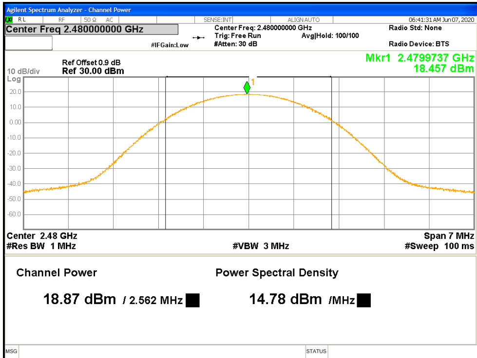
Figure 4: BLE Maximum Conducted Output Power at 2480 MHz
