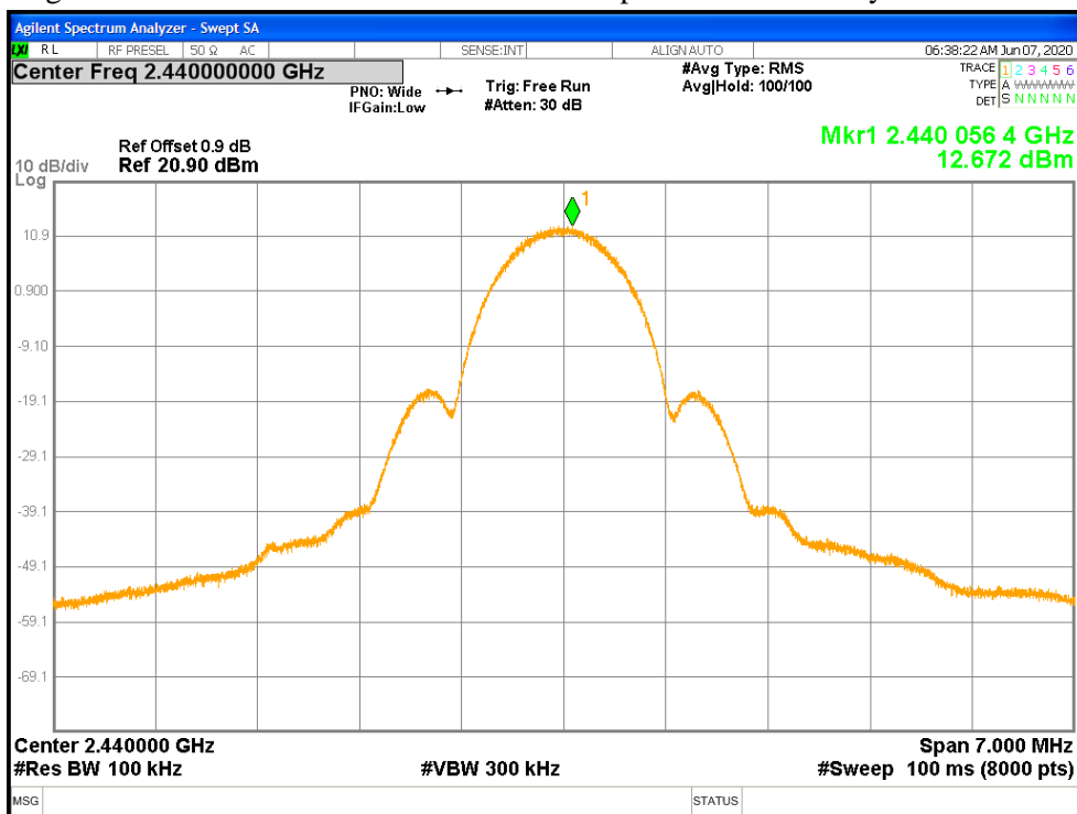
Figure 12: BLE Maximum Power Spectral Density-2440 MHz
