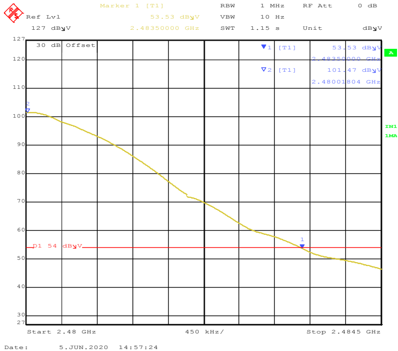
Figure 27: Band-edge-2480 MHz-H-Avg
