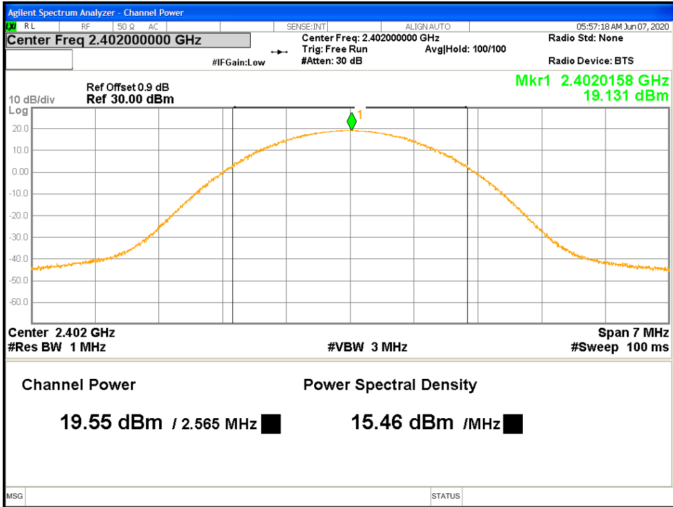
Figure 2: BLE Maximum Conducted Output Power at 2402 MHz
