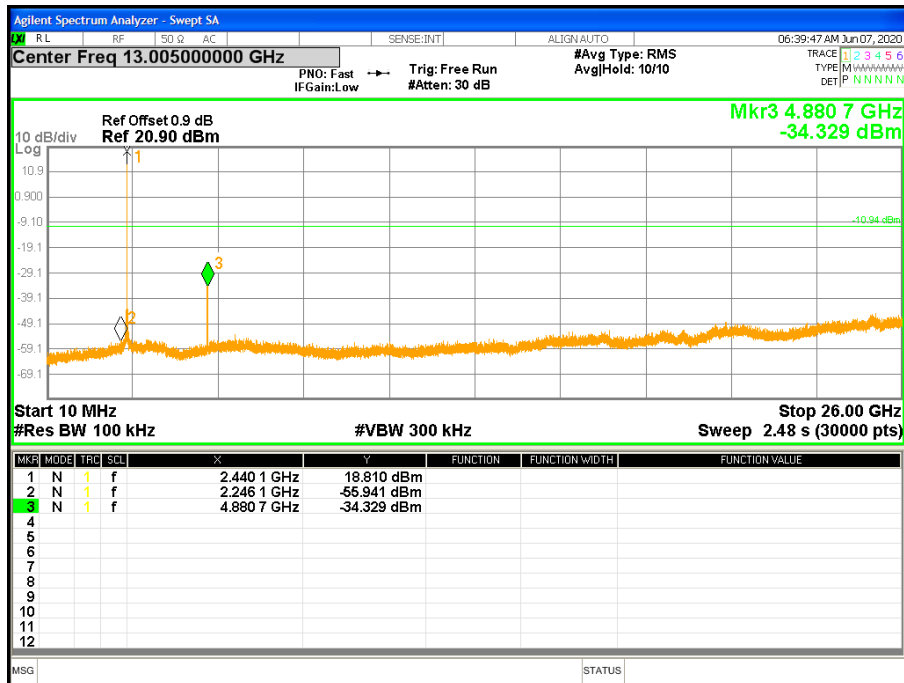
Figure 17: BLE Out of band Emission at 2440 MHz
