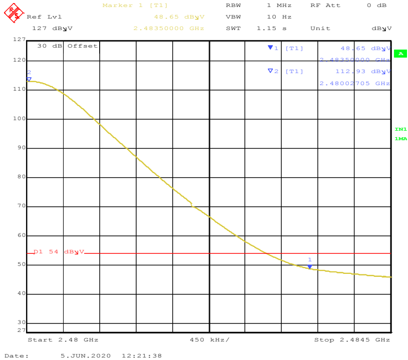
Figure 25: Band-edge-2480 MHz-V-Avg
