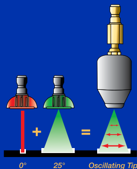
Oscillating Tip (5000 psi) Part No. 198013
