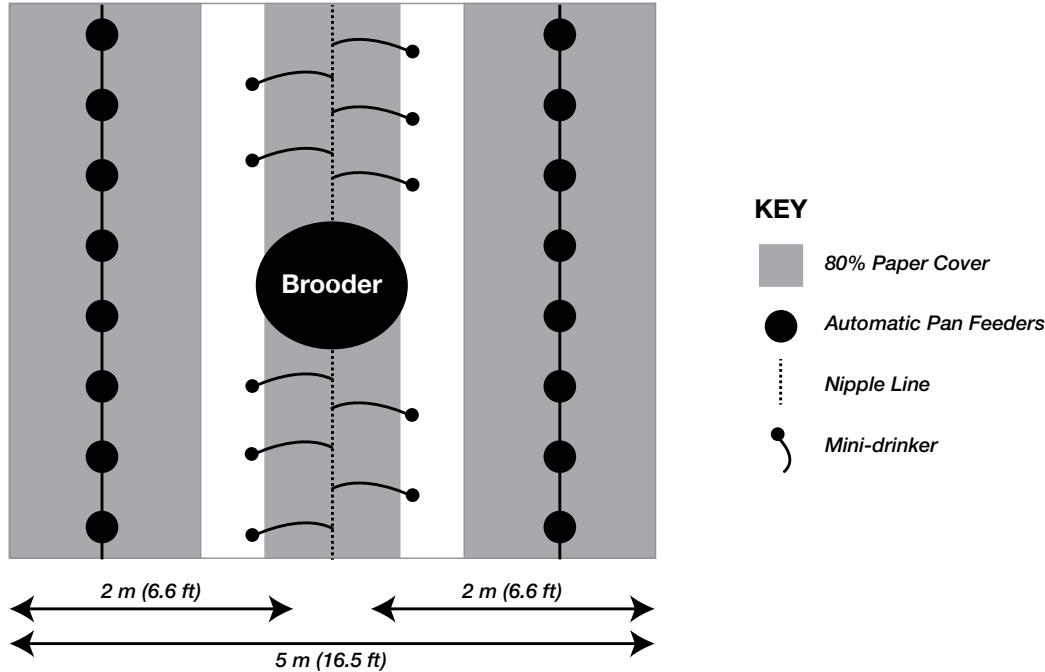
Figure 9: Typical spot brooding layout (1,000 chicks).
