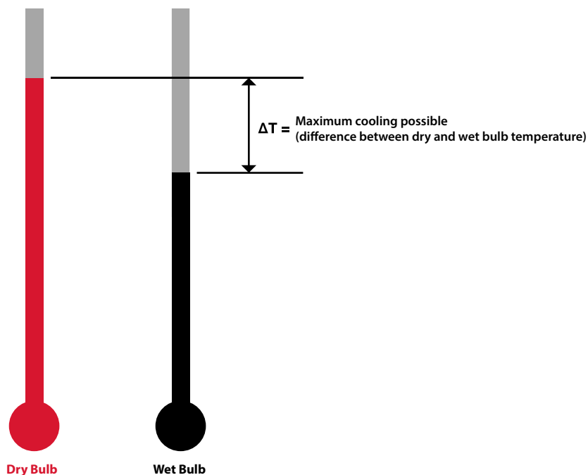
Figure 43: Maximum cooling possible during evaporative cooling is about 0.75 of the difference between dry and wet bulb temperature.
