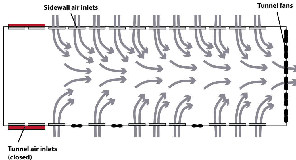
Figure 38: Typical air movement during transitional ventilation.
