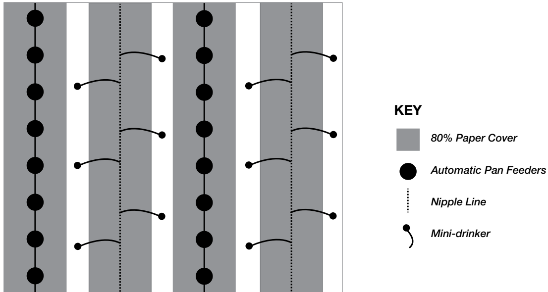
Figure 11: Typical layout of a whole-house brooding system.
