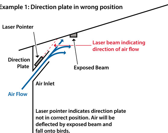
Figure 35: Using a presentation laser to determine if the air direction plate is positioned correctly. A simple laser pointer can be used to provide a visual reference of direction of airflow in to the house. The direction plate can then be set to ensure that airflow bypasses any ceiling obstructions.
