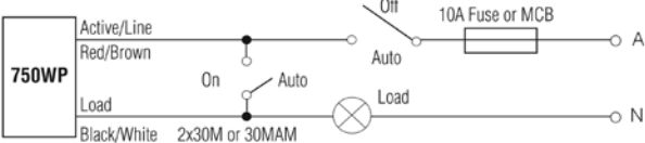
1c) ON, OFF or AUTOMATIC Operation using a 3 position switch
