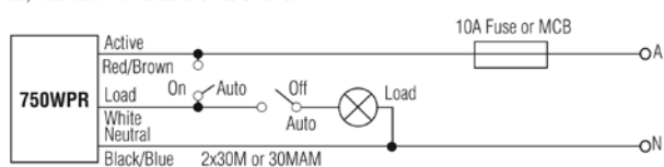
2b) Automatic with manual override ON or OFF
