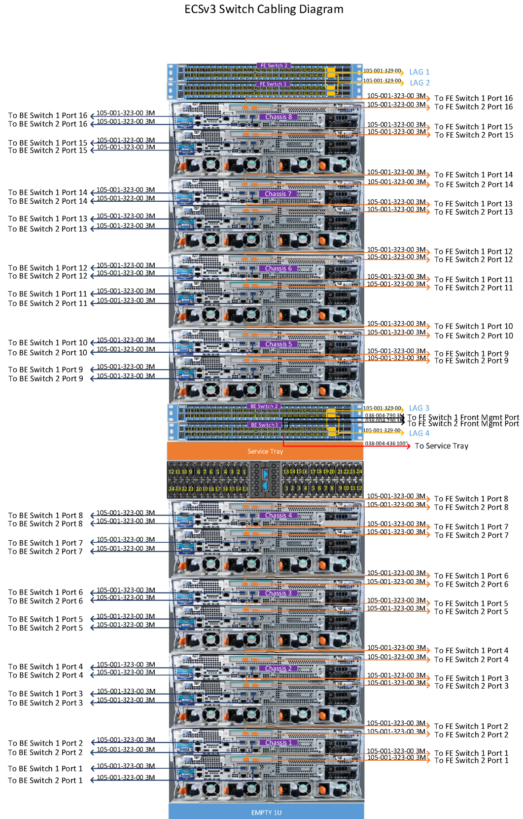
Figure 95 EX3000D network cabling
