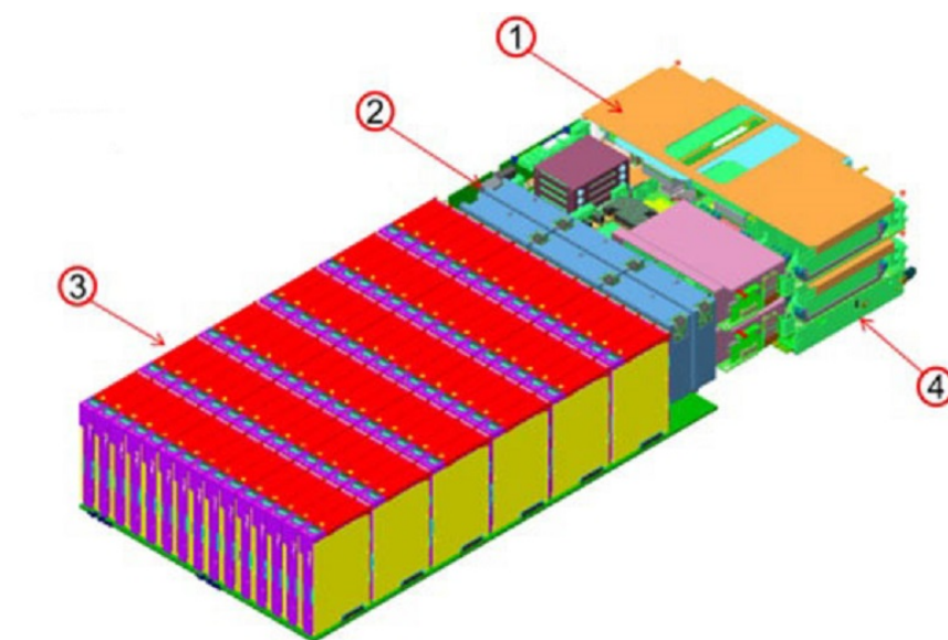
Figure 70 EX3000 internal chassis view
