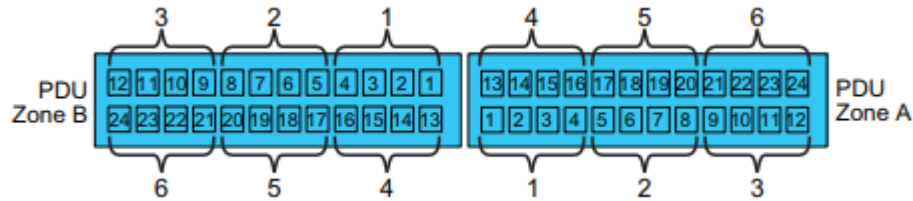
Figure 76 PDU outlet numbers
