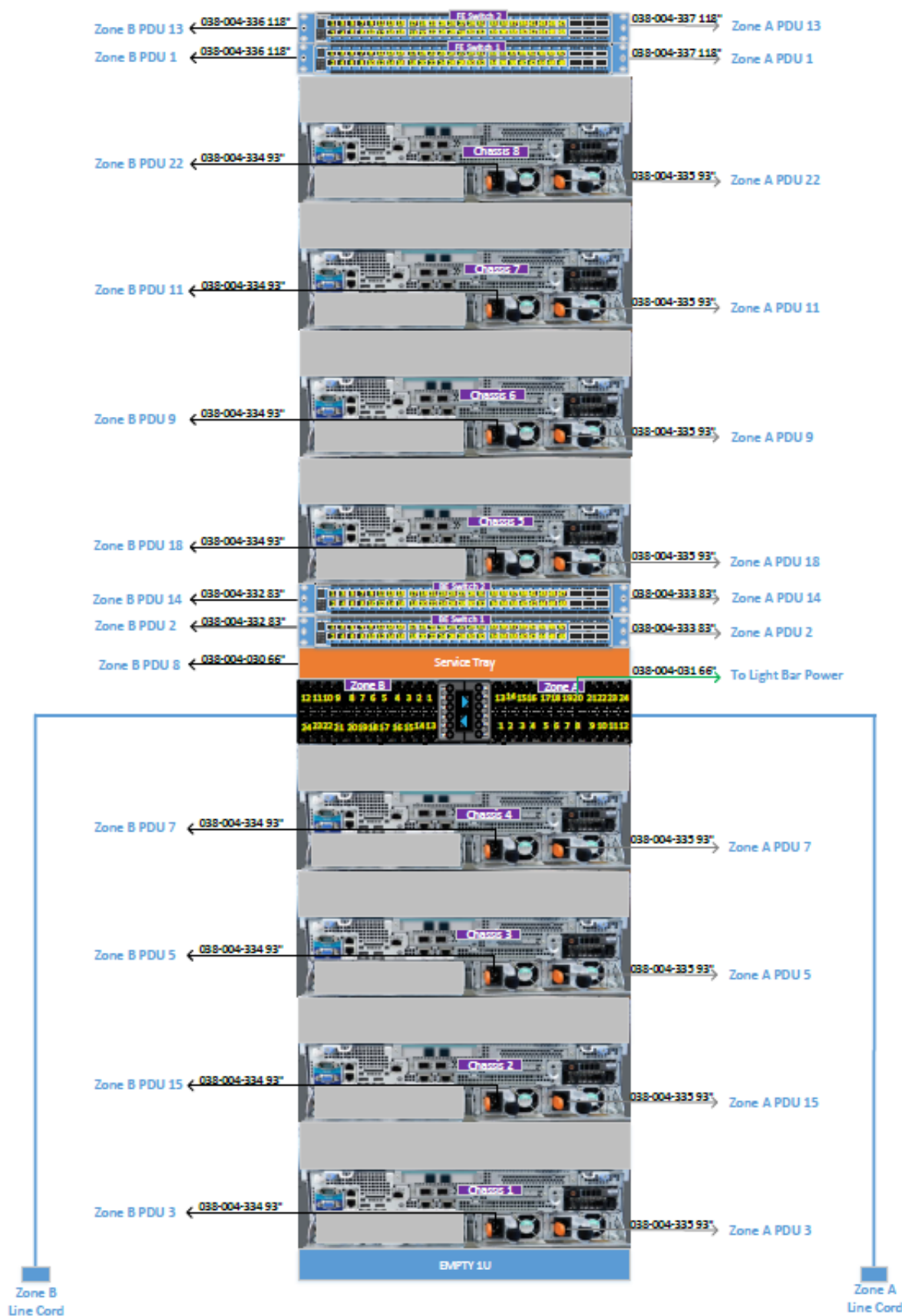
Figure 83 EX3000S three-phase WYE AC power cabling
