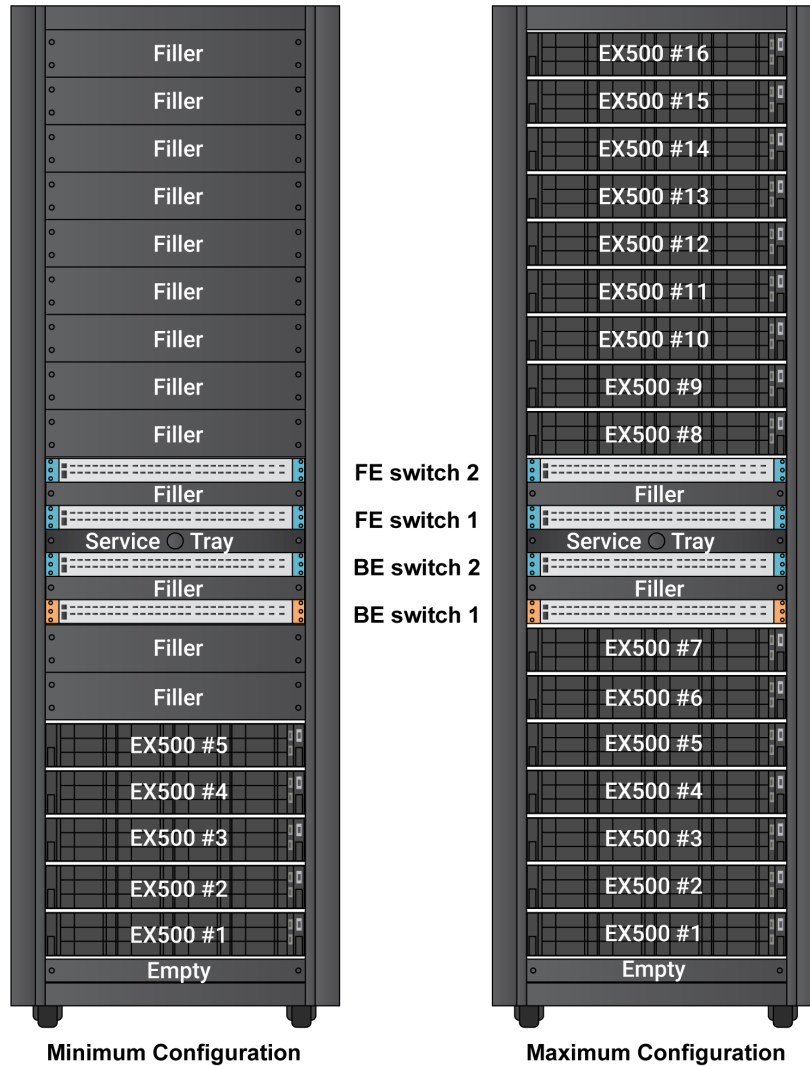
Figure 7 EX500 minimum and maximum configurations
