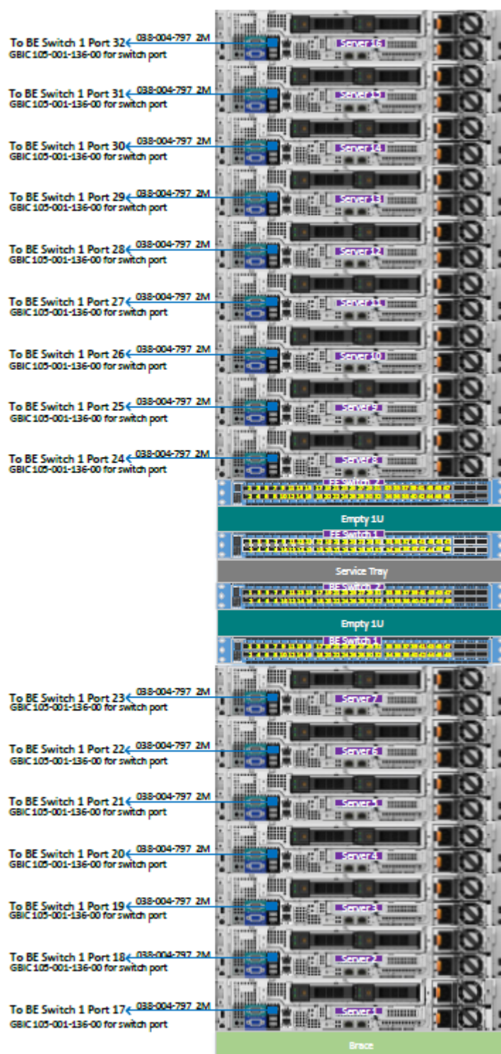
Figure 19 iDRAC cabling
