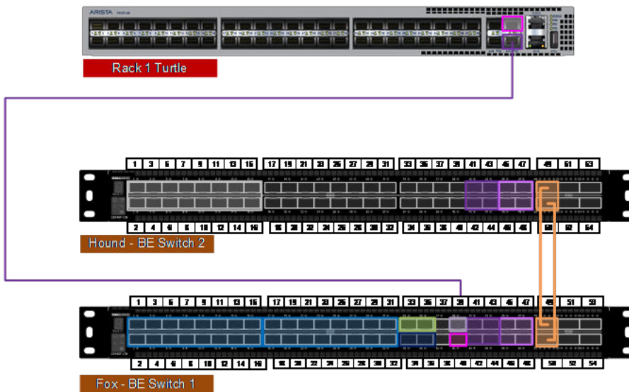
Figure 61 Inter-rack switch connectivity - linear topology (daisy-chain) between an EX-Series rack and a Gen2 U-Series, D-Series, or C-Series rack
