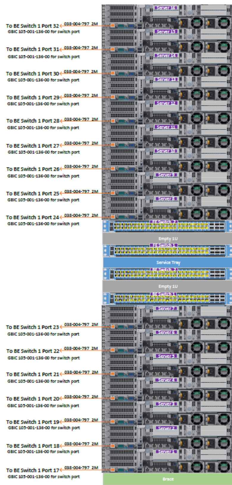
Figure 50 iDRAC cabling
