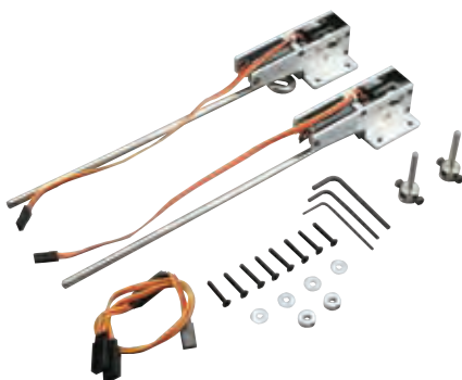
60-120 85-Degree Strut Ready Main Electric Retracts EFLG510
