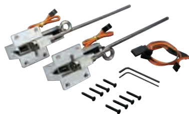
60-120 95-Degree Electric Rotating Retracts EFLG520
