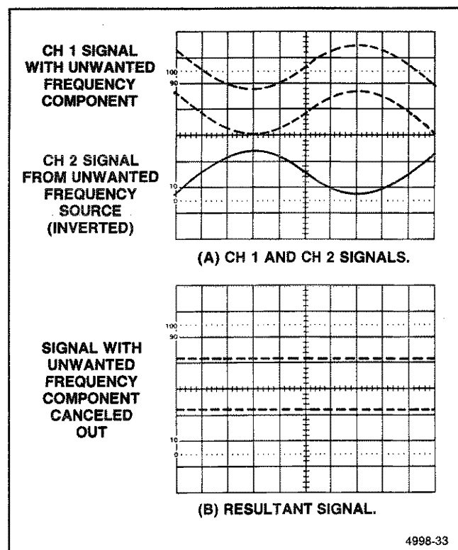
Figure 6-4. Common-mode rejection.
