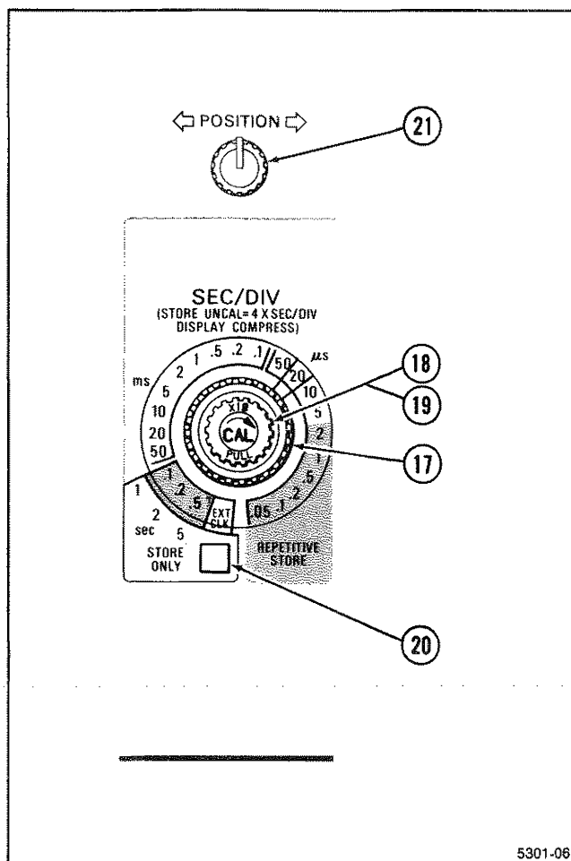
Figure 3-3. Horizontal controls.
