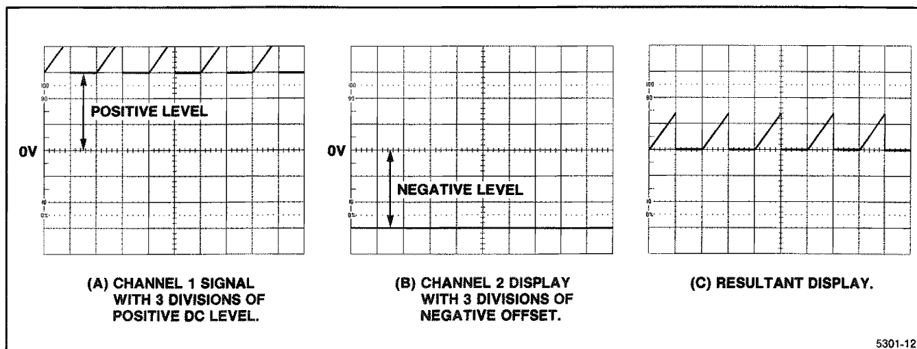
Figure 6-3. Algebraic addition.
