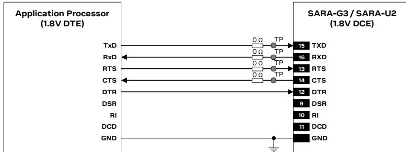
Figure 68: UART interface application circuit with partial V.24 link (6-wire) in the DTE/DCE serial communication (1.8 V DTE)
