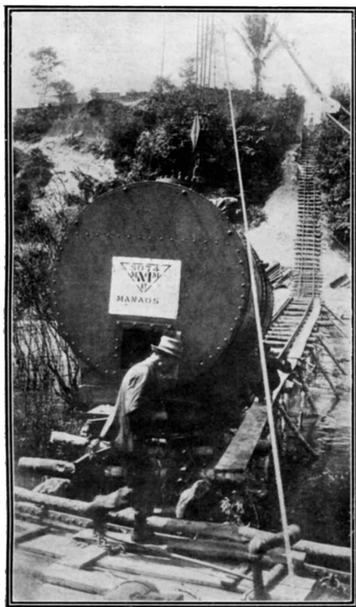
Hoisting Boiler up the Incline Plane, Manaos.
