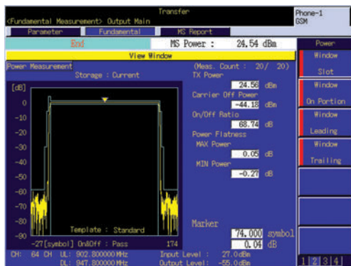
Entire Time Slot of GMSK Modulation
