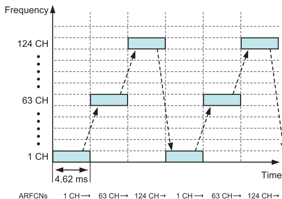
Example of Hopping Frequency
