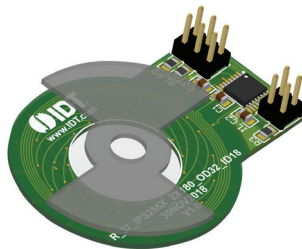
2 Pole-Pairs
