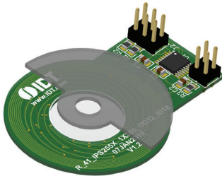
1 Pole-Pair
