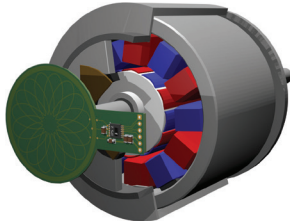
End-of-Shaft
