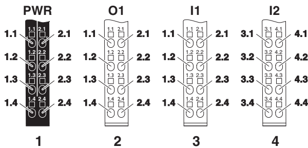
Figure 3 Terminal point assignment
