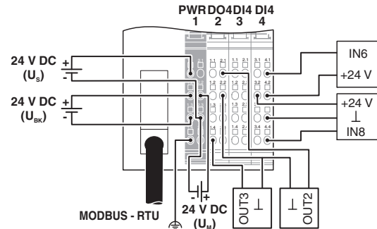
Figure 4 Connection example
