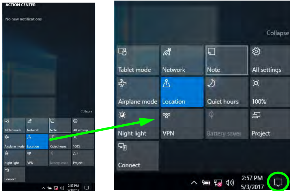
Figure 1 - 17 - Action Center
