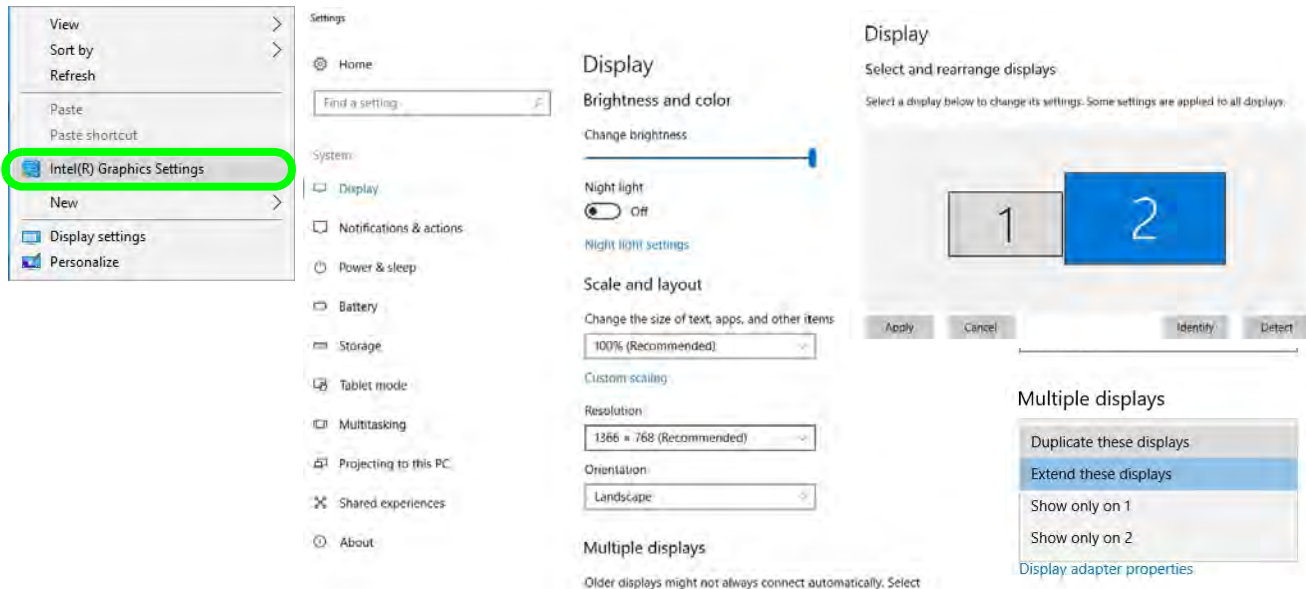
Figure 1 - 19 - Display Settings
