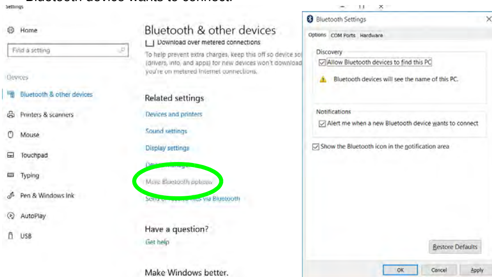
Figure 6 - 14 Bluetooth Settings
