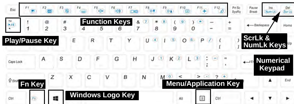
Figure 1 - 4 - Keyboard
