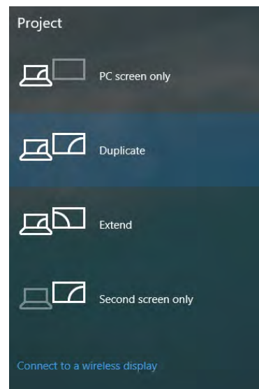
Figure 1 - 18 - Project (Devices)
