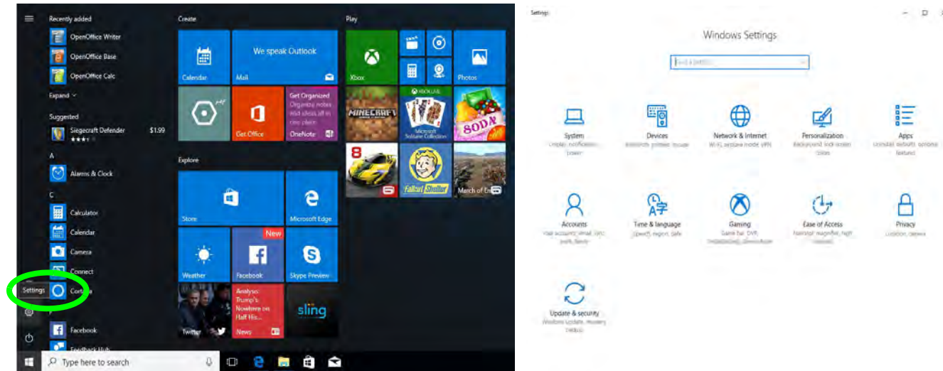
Figure 1 - 15 - Settings
