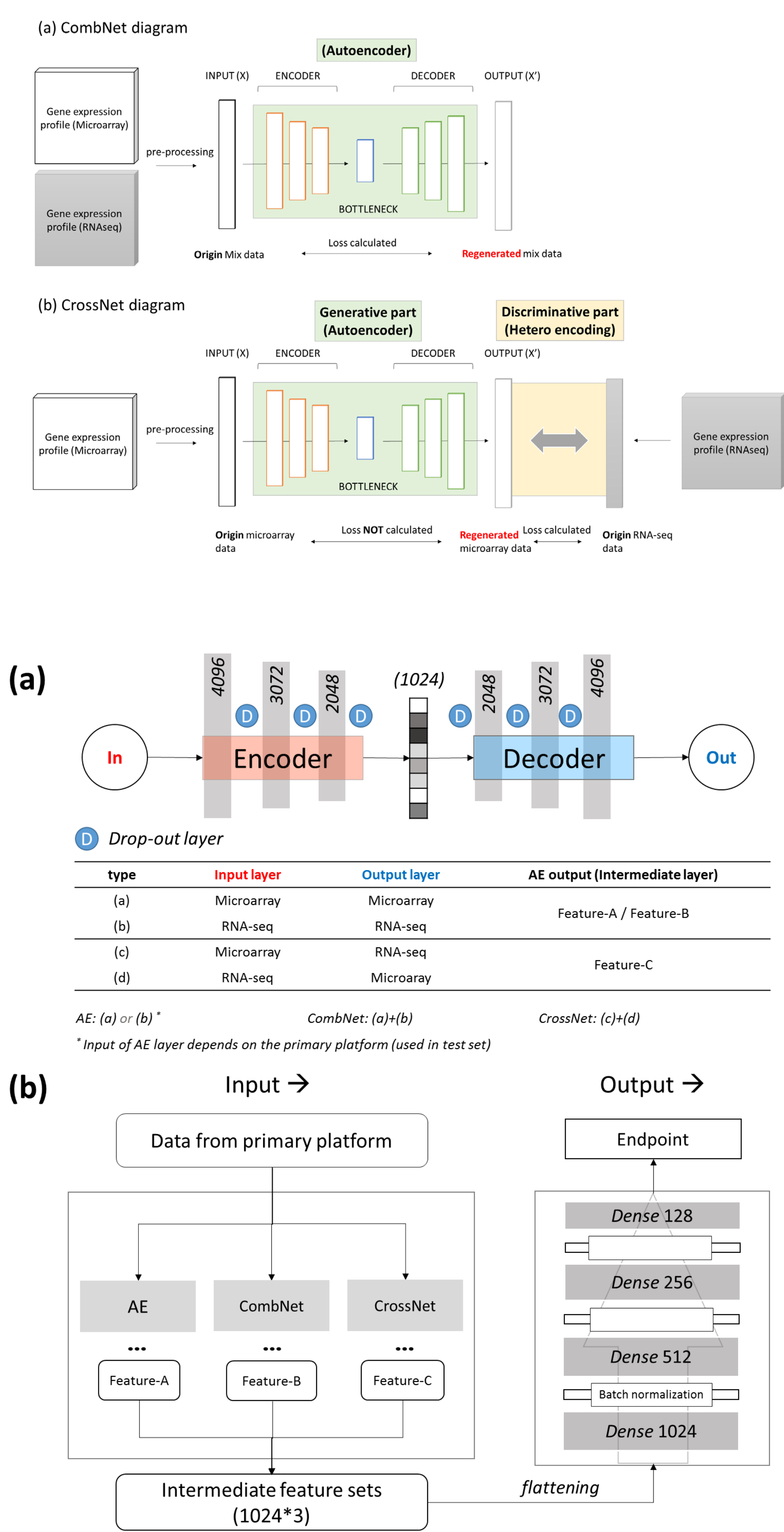
Figure 2. HetEnc overview. (a) feature representation model architecture and three different encoding networks (AE, CombNet and CrossNet) used in the study; (b) feature extraction and 6-DNN structure in the modeling step.
