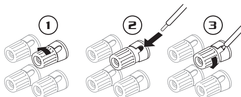
Banana Connector
