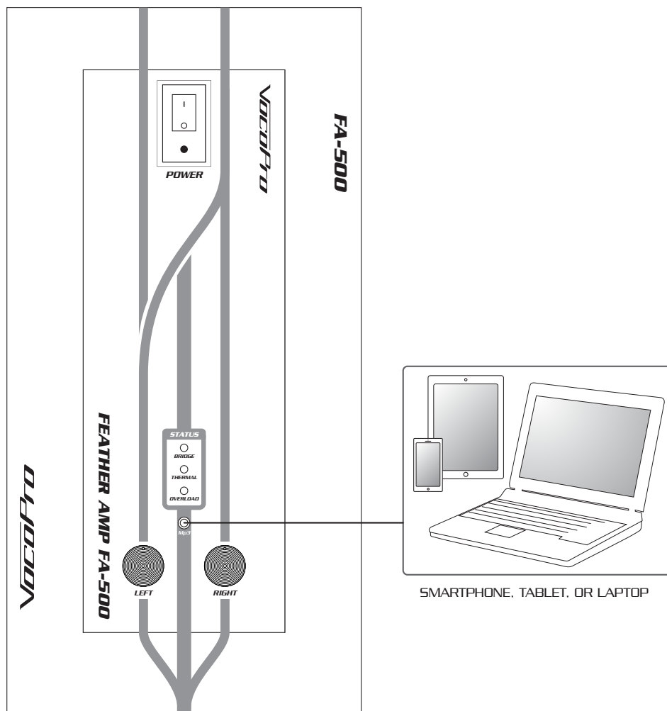
Top Panel
