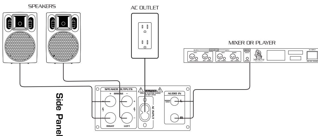
Connection Diagram 1.5
