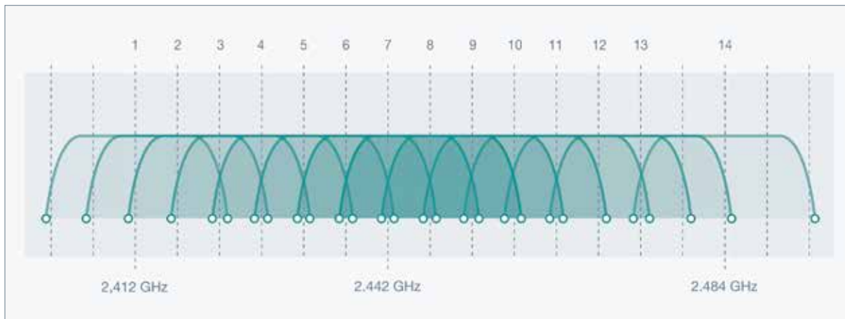
Figure 24: Channel designation in 2.4GHz band according to IEEE 802.11
