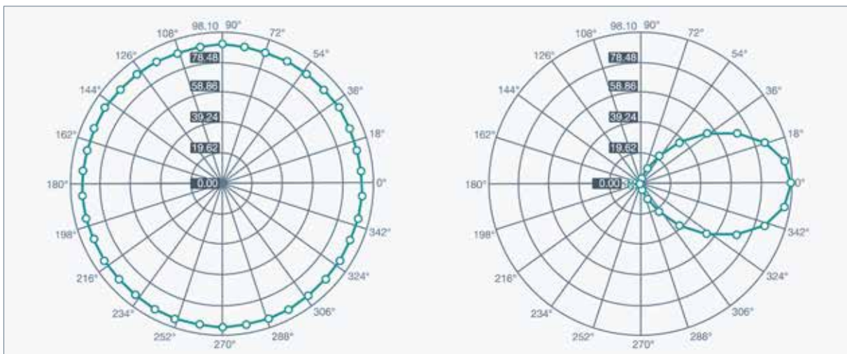
Figure 18: Radiation pattern of omnidirectional and directional antennas
