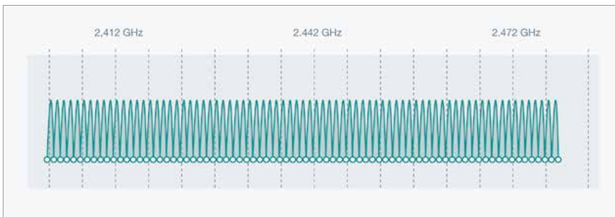
Figure 25: Channel designation in 2.4GHz band according to IEEE 802.15.1
