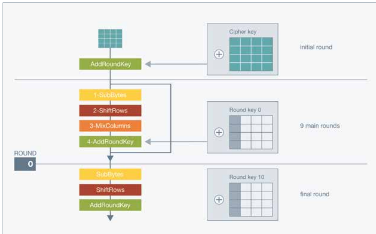
Figure 21: AES encryption process
