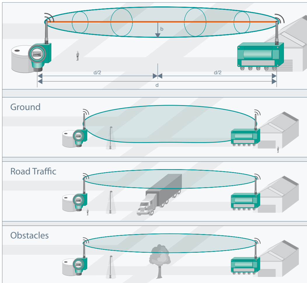
Figure 11: Fresnel zone and possible disruptions
