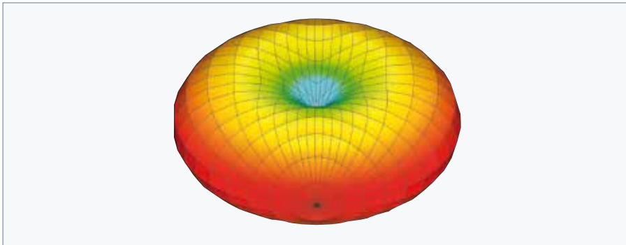
Figure 15: Radiation pattern of undisturbed dipole antenna
