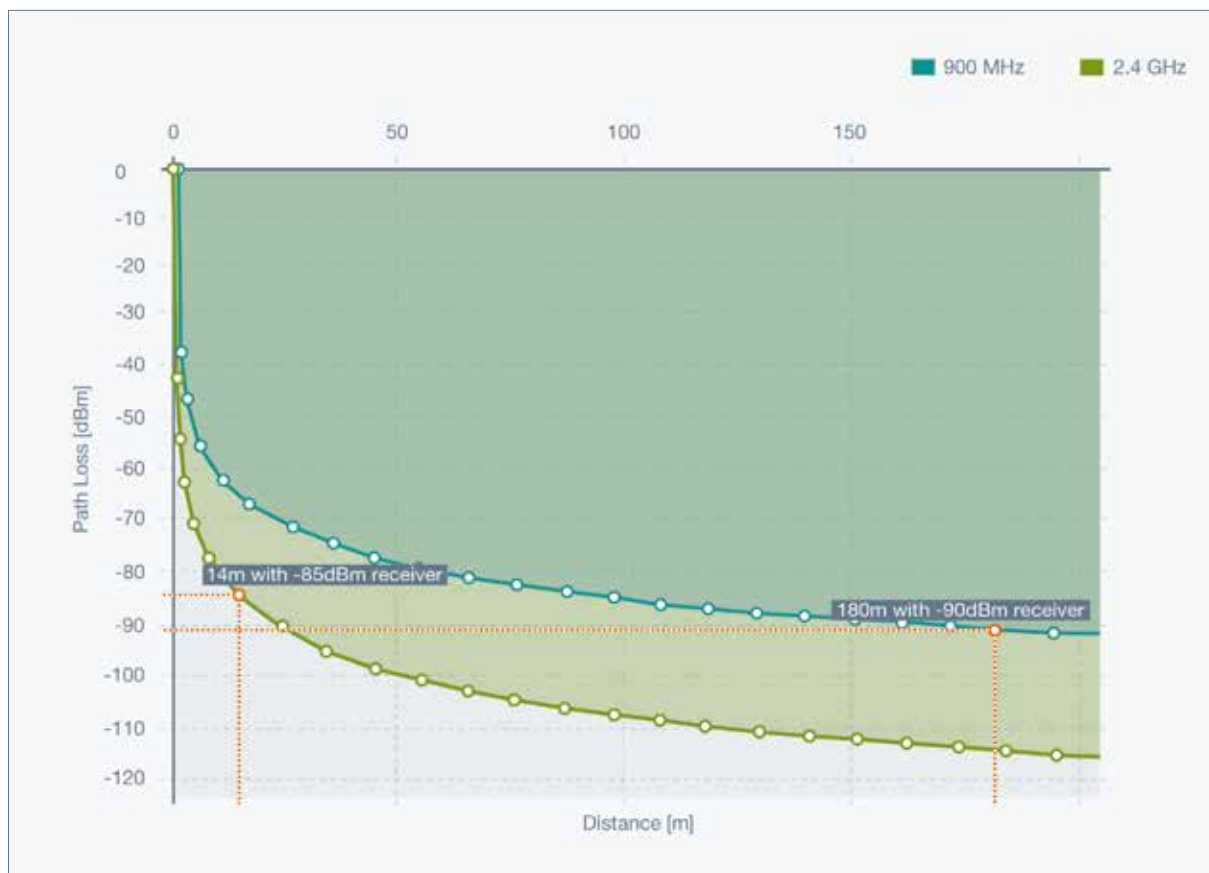
Figure 5: Real propagation in a shadowed urban environment (path loss exponent of 3.7)
