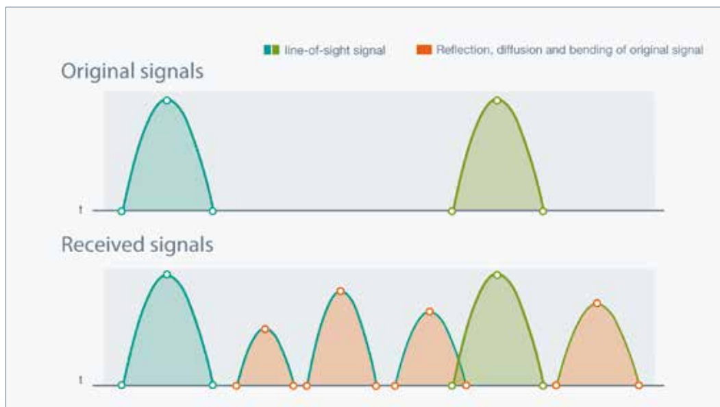
Figure 10: Receipt of the original signal and its reflections, bendings, and diffusions
