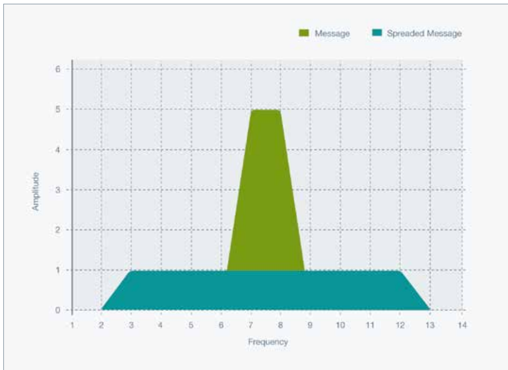
Figure 14: Direct sequence spread spectrum
