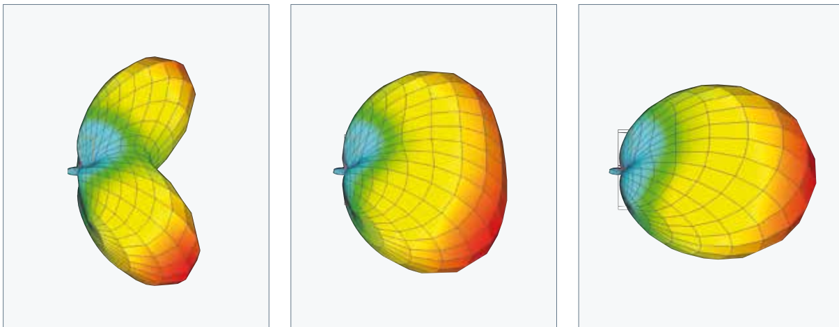
Figure 16: Radiation pattern of dipole with reflective plane in different distances
