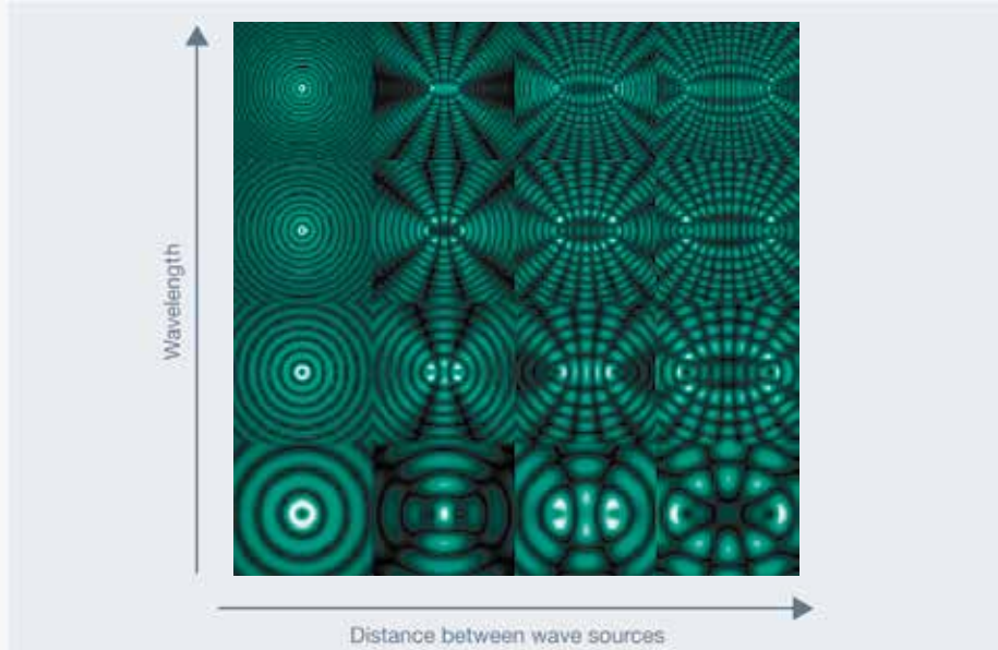
Figure 9: Interference of two circular waves, dark areas destructive, light areas constructive interference (Author: Florian Marquardt (Ludwig-Maximilians-Universität München))
