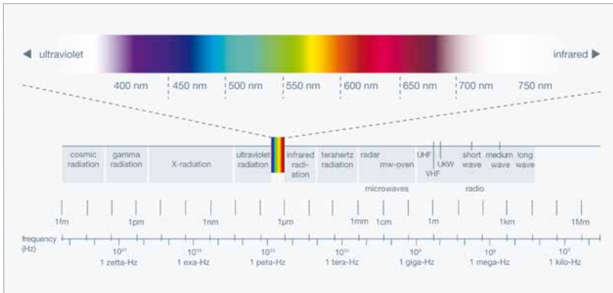
Figure 1: Electromagnetic spectrum
