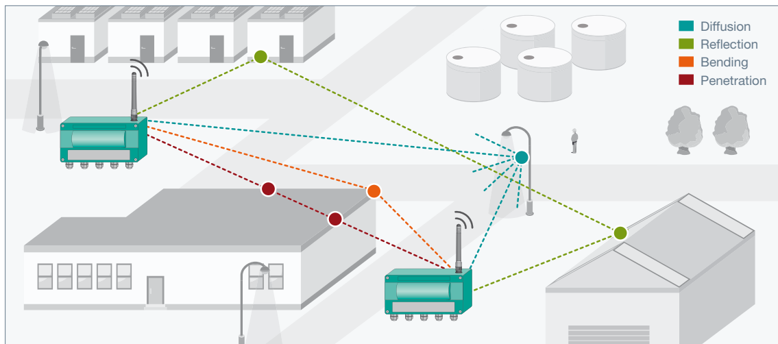
Figure 6: Diffusion, reflection, bending, and penetration of obstacles
