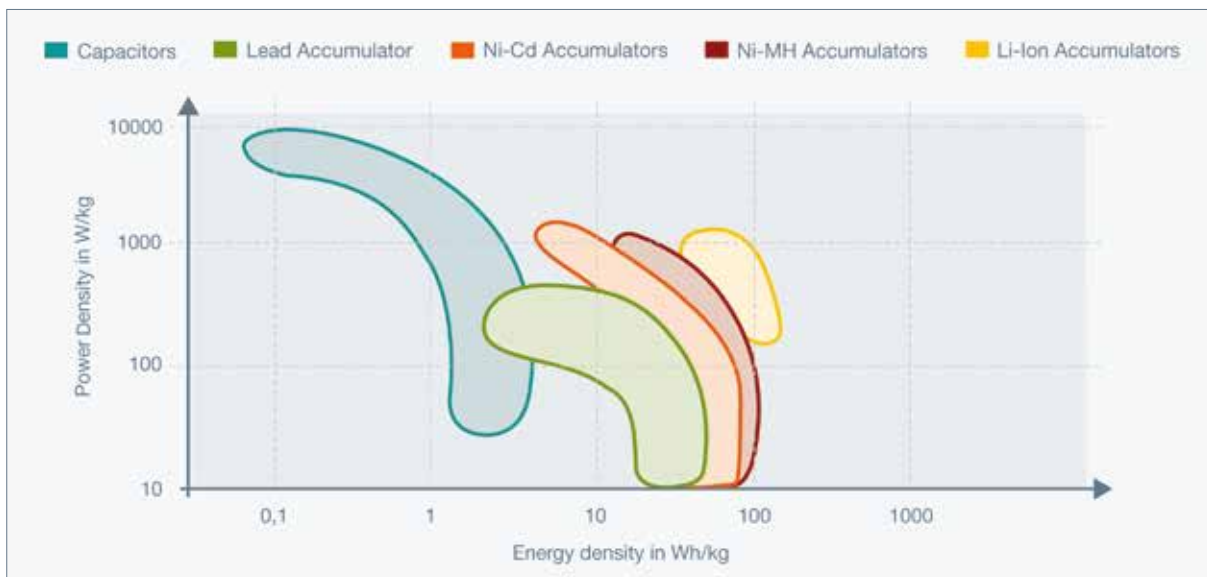
Figure 19: Power and energy density of different battery-types.
