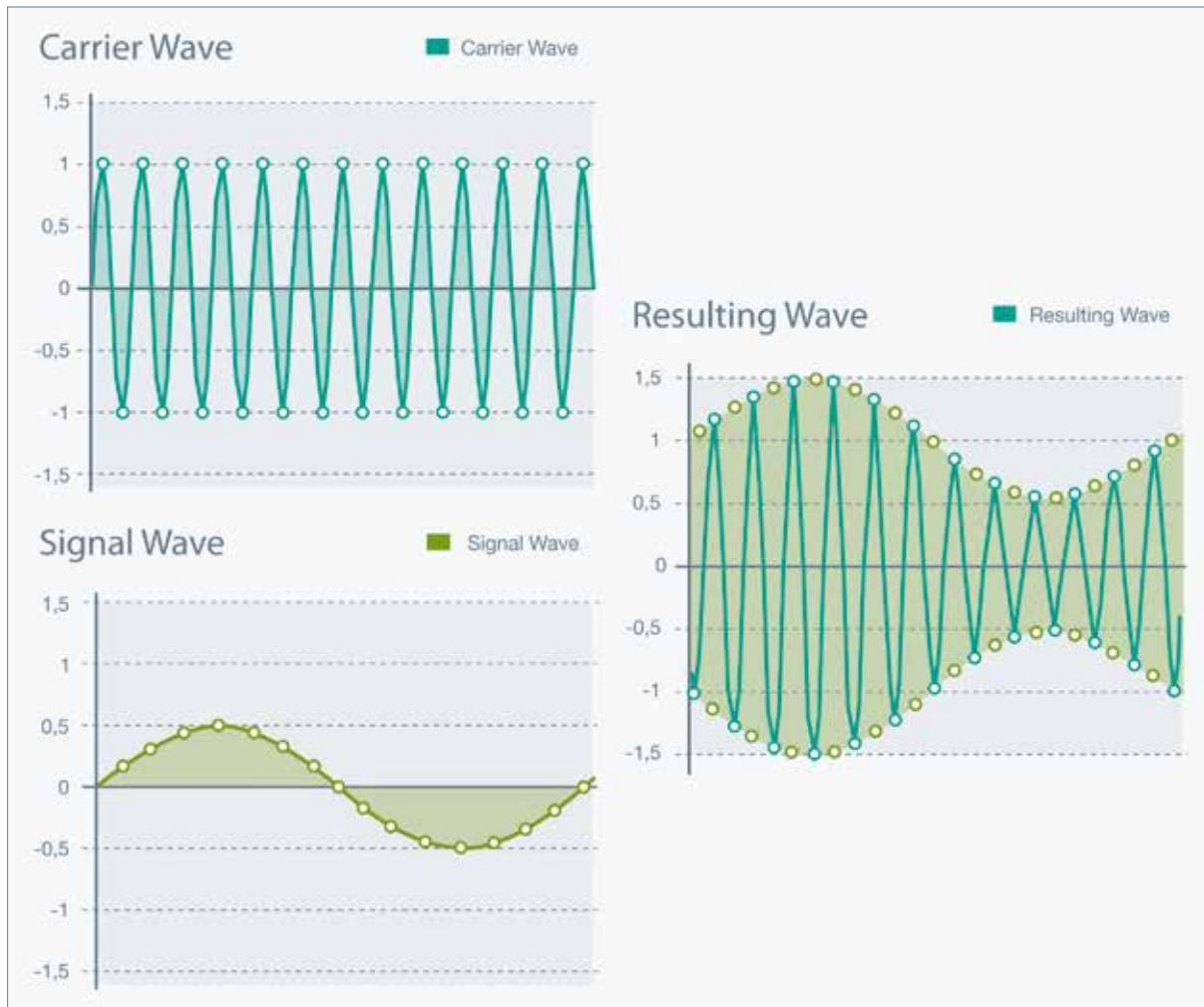
Figure 12: Amplitude modulation – carrier wave, Signal wave, and resulting wave
