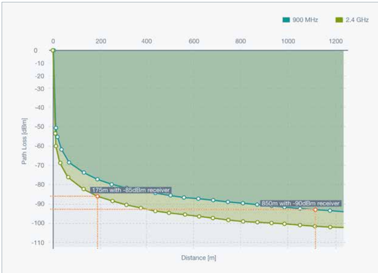
Figure 4: Theoretical free space propagation
