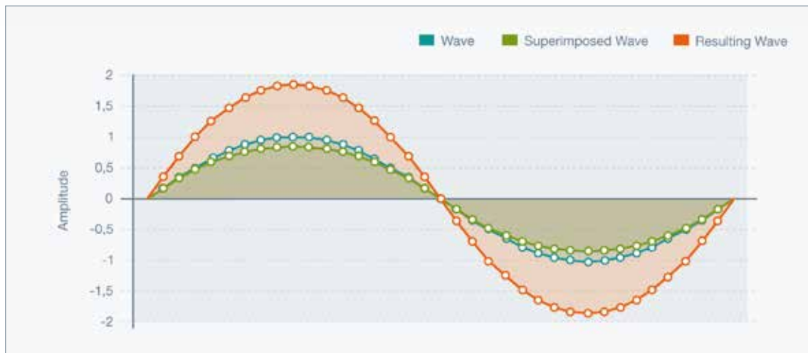
Figure 7: Positively superimposed wave, constructive interference
