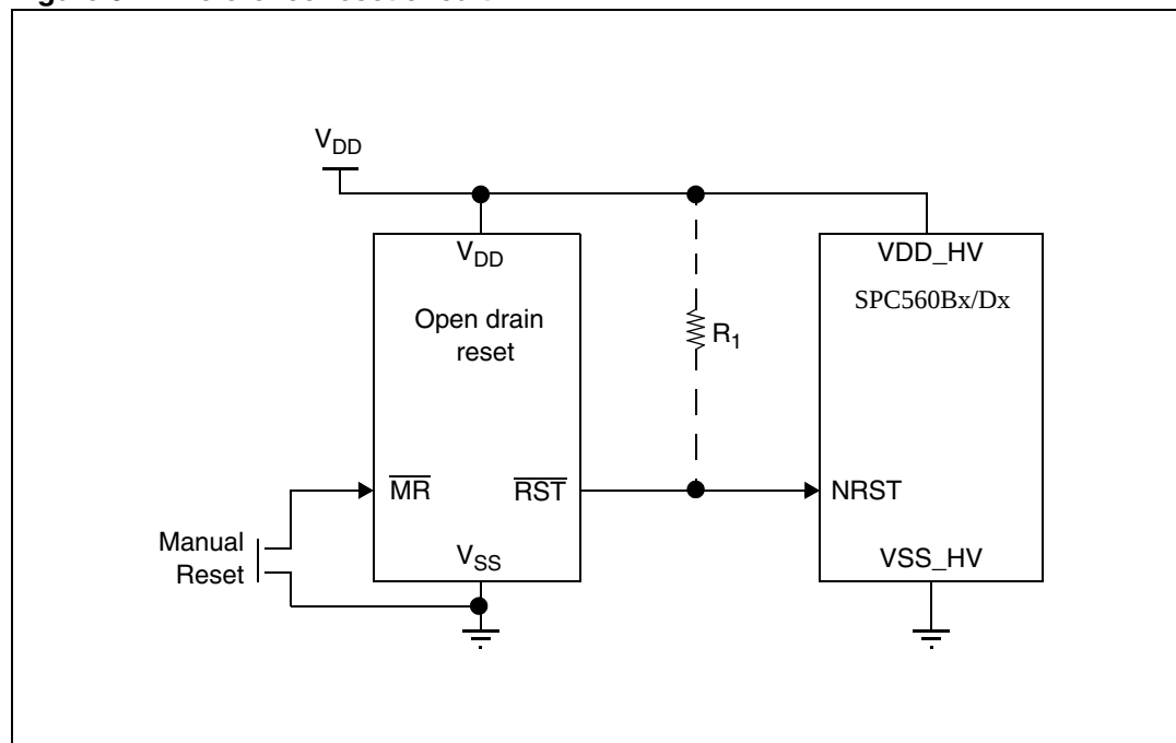
Figure 6. Reference reset circuit
