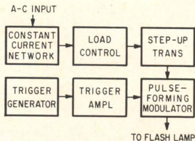
BASIC power supply system comprises power supply proper (above) and trigger circuits that operate pulse modulator (below)—Fig. 1
