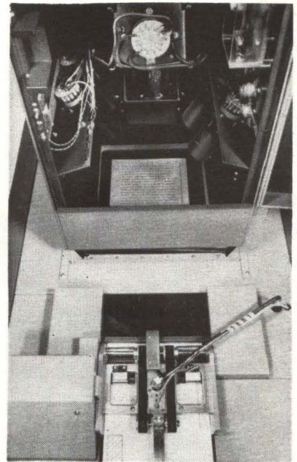
VACUUM-ASSISTED mechanical equipment smooths out document and positions it under special flying-spot scanner (above)
