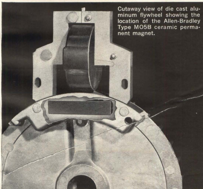
Allen-Bradley Type MO5B magnet used in Briggs & Stratton engine.
