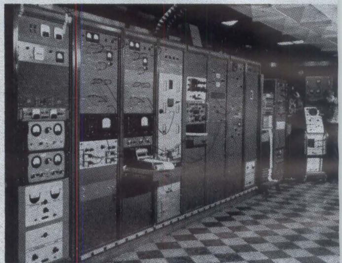
RECEIVER room, containing i-f section and some data processing equipment, is connected by 1,400 feet of coaxial cable to receiver front end located in antenna house
