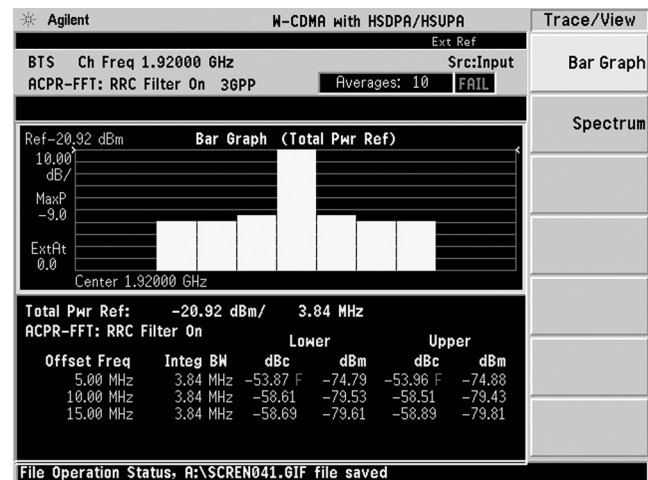
Figure 2. Multi-offset ACPR
