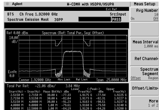
Figure 4. Spectrum emission mask
