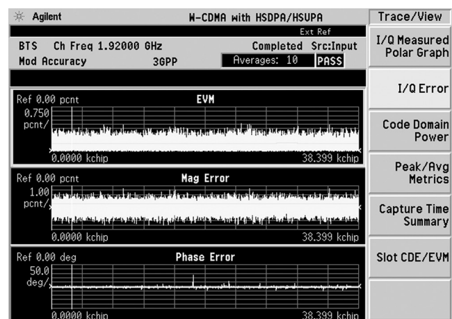
Figure 16. Error plots of magnitude error, phase error, and EVM over 15 slots
