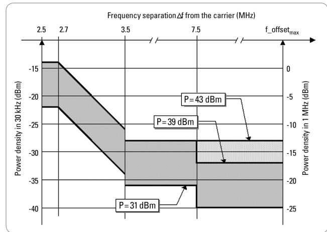
Figure 3. W-CDMA specification for spectrum emission mask (from TS25.104 v6.17.0 (2008-03))
