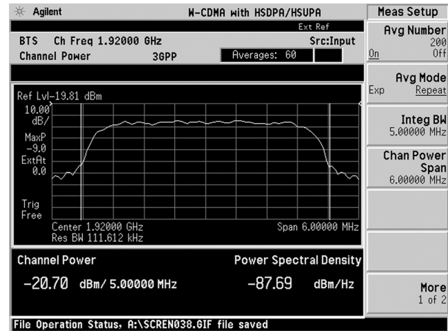
Figure 1. Channel power
