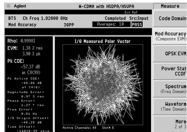
Figure 15. Modulation accuracy of HSDPA signal
