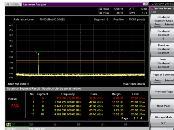
Spectrum Analyzer Spurious Emission Function
