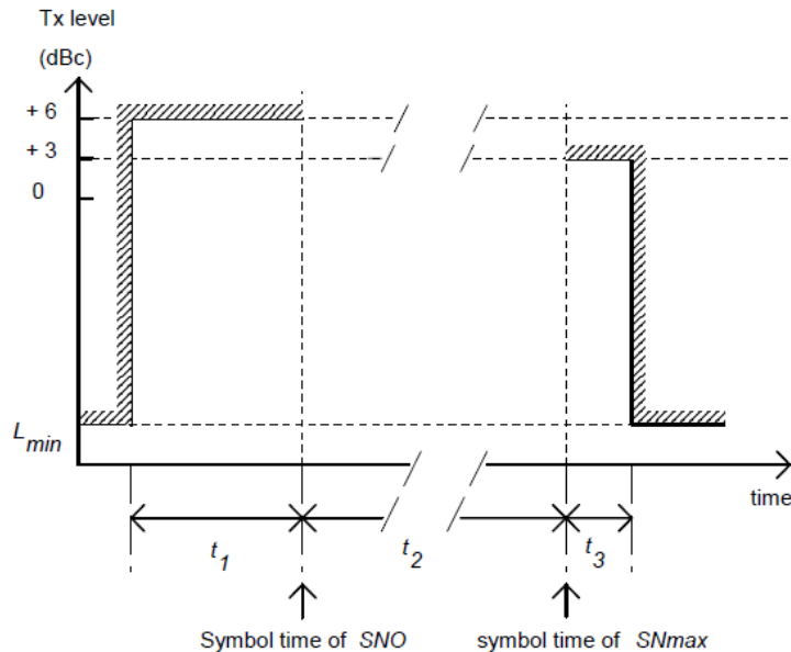
Figure 6.3: Transmit level versus time mask
