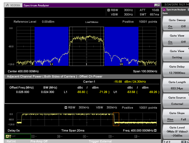
Ramp-down period Measurement Example
