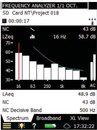
Fig.10.6 Displaying a Noise Curve together with the L_{Zeq} spectrum
