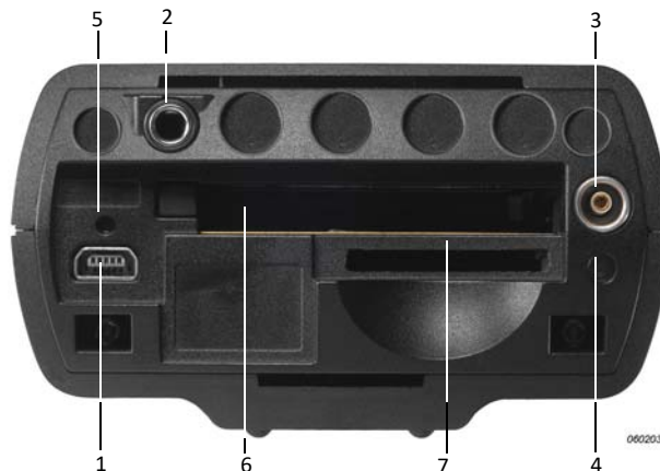
Fig. 2.2 Connector panel of 2250 Light for G1 – 3 analyzers
