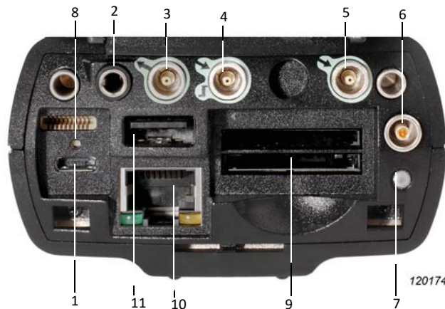
Fig. 2.3 Connector panel of 2250 Light for G4 analyzers
