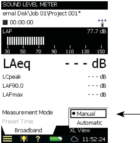
Fig.3.3 Setting the measurement mode
