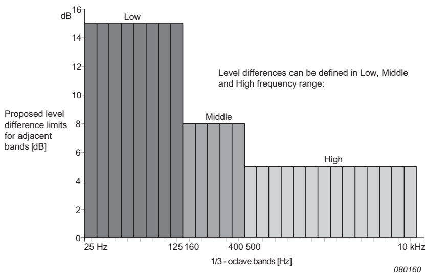
Fig. 13.1 Definition of frequency ranges and level differences
