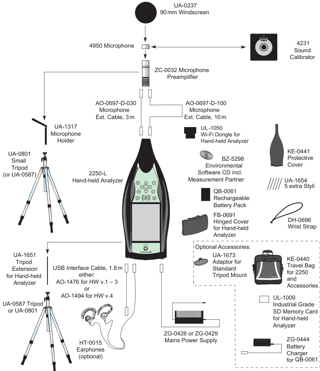
Fig. 2.4 2250 Light – hardware overview
