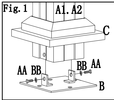
Fig.1: Put base cover (C) into post (A1, A2), then attach base (B) to post (A1, A2) with Bolt (AA) and washer (BB).
