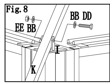
Fig.8: Attach Curved beam down tube (K) to Posts (A1, A2) with Bolt (DD), Washer (BB) and Nut (EE).
