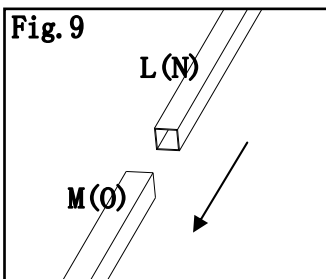
Fig.9: Insert Long middle beam (L) into Middle beam down tube (M). Repeat this Step for Short middle beam (N) and Short middle beam down tube (O).
