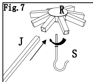
Fig.7: Insert Curved beam (J) into Large top connector (R), then fix hook (S) onto large top connector (R).
