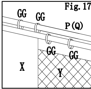
Fig.17: Hang mosquito nets (Y) and curtains (X) onto long mosquito net rails (P) and short mosquito net rails (Q) with plastic rings (GG).
