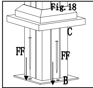
Fig.18: Lift base cover (C), secure the whole gazebo to the lawn by inserting stakes (FF) in the holes of each base.
