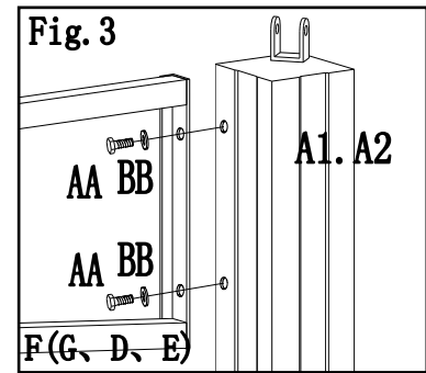
Fig.3: Attach Long side Long beam (F) to Post (A1) with Hex Bolt (AA) and Washer (BB), Repeat this step for Long side short beam (G), short beam. (D, E).
