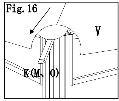
Fig.16 : Spread out Big canopy (V) , Attach on the corners of Curved beam down tube (K), Middle beam down tube (M) and Short middle beam down tube (O).
