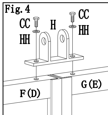
Fig.4: Attach Middle beam down connector (H) to Long side Long beam (F) Long side short beam (G) with Bolt (CC) and Washer (HH). Repeat this step for short beam (D, E).
