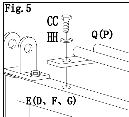
Fig.5: Attach Long mosquito net rail (P) to Long side beam (F,G) with Bolt (CC) and Washer (HH). Repeat this step for short beam (D, E).
