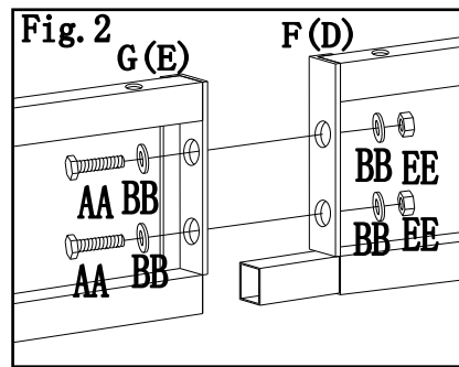
Fig.2: Insert long side long beam (F) into long side short beam (G), then fix with bolt (AA), washer (BB) and nut (EE). Repeat this step for short beam (D, E).
