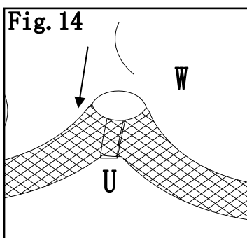
Fig.14: Put small canopy (W) on small top, then attach four corners of small canopy to small top curved beam (U).
