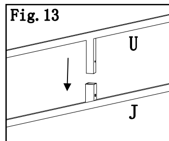
Fig.13: Insert small top curved beam (U) into Curved beam (J).
