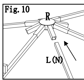
Fig.10: Insert Long middle beam (L) into Large top connector (R). Repeat this step for Short middle beam (N).
