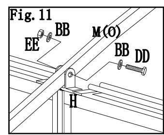
Fig.11: Fix Middle beam down tube (M) and Short middle beam down tube (O) onto Middle beam down connector (H) with Bolt (DD), Washer (BB) and Nut (EE). Put Big canopy (V) on Big Top, but do not spread it now.
