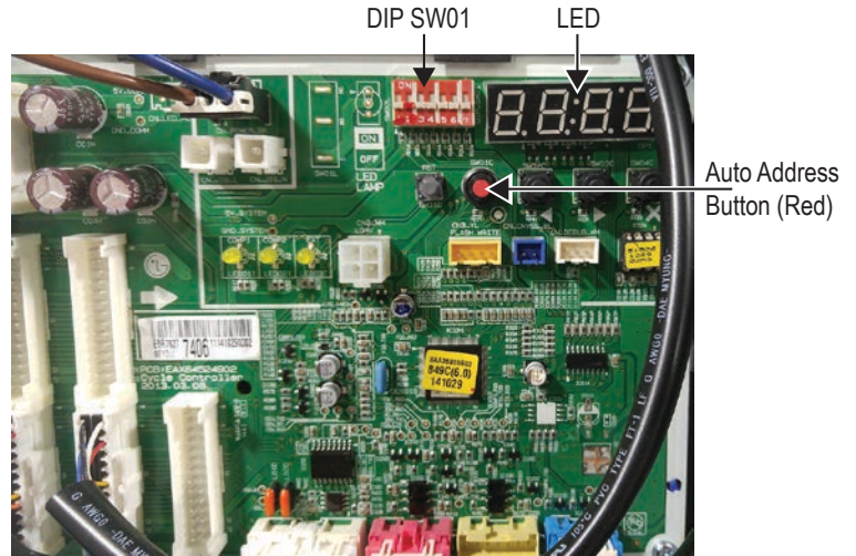
Figure 80: Auto Address Button Location.
