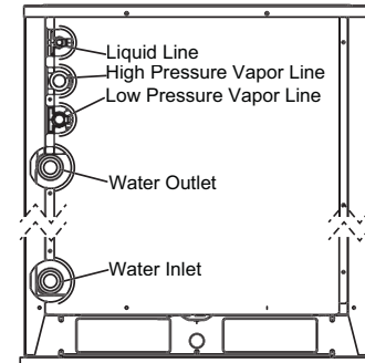
Figure 46: Water Source Unit Front Panel.
