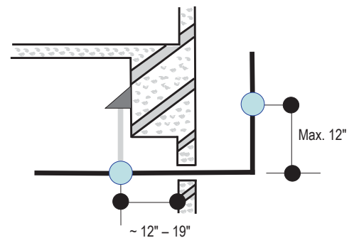
Figure 31: Typical Pipe Support Location—Change in Pipe Direction.
