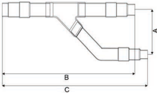
Figure 5: Y-branch dimensions (See Table 20).
