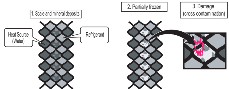
Figure 64: Potential Heat Exchanger Damage.
