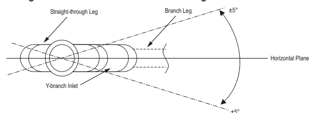
Figure 22: Y-Branch Horizontal Configuration End View.
