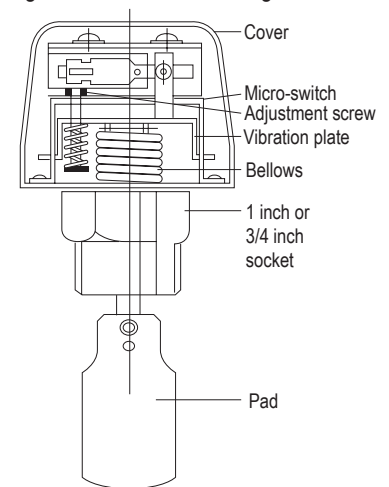
Figure 65: Flow Switch Diagram.
