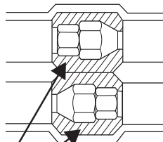
Figure 53: Typical Refrigerant Flare Fitting Insulation Detail.
