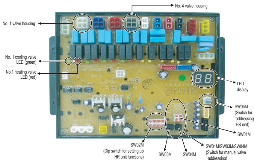
Figure 83: Heat Recovery Unit PCB Dip Switches.
