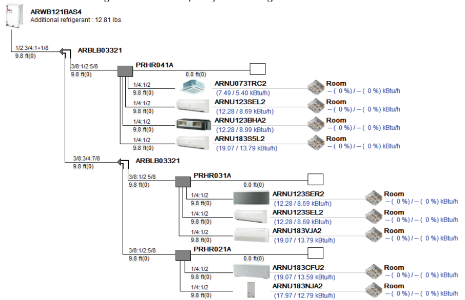
Figure 19: LATS Pipe System Design Tool in Tree Mode.
