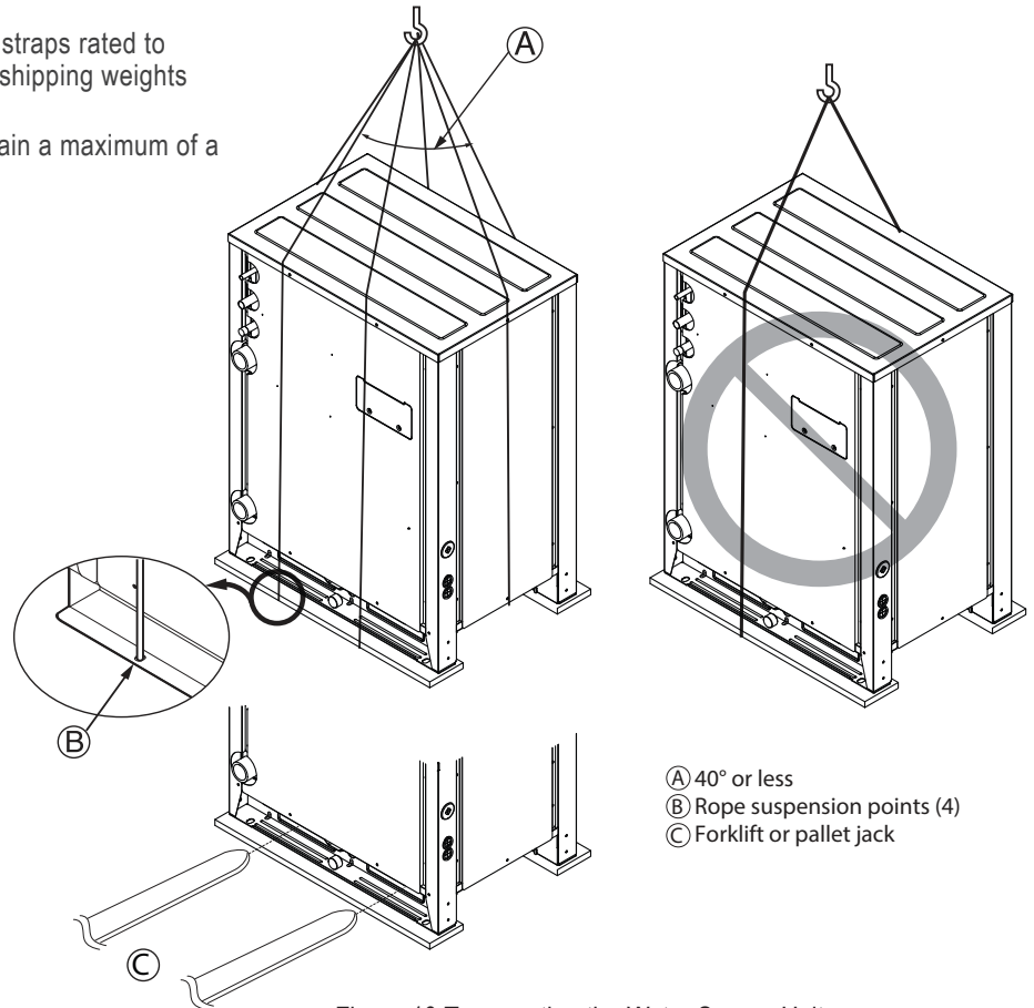
Figure 10: Transporting the Water Source Unit.
