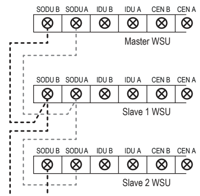
Communications Between WSUs
