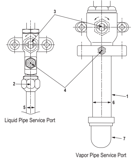
Figure 47: Service and Schrader Valve Detail.
