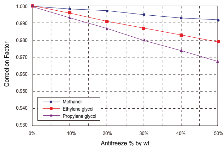
Figure 62: Cooling Capacity Correction Factor Chart.
