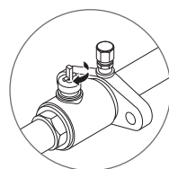
Figure 48: Service Valves - Open and Closed Positions.
