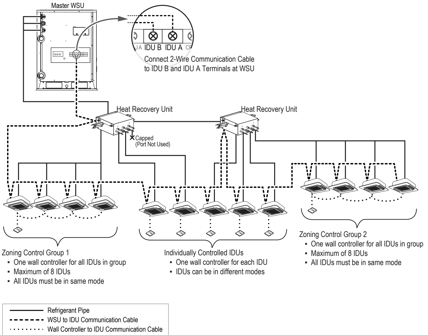
Figure 75: Typical IDU Zone Control Connections
