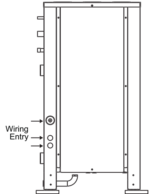
Figure 69: Access Holes for Power Wiring and Communication Cable Connections.
