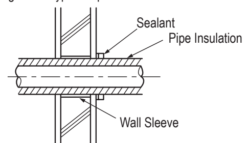
Figure 35: Typical Pipe Penetration.
