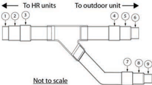
Figure 8: Y-branch Dimensions (See Table 27).
