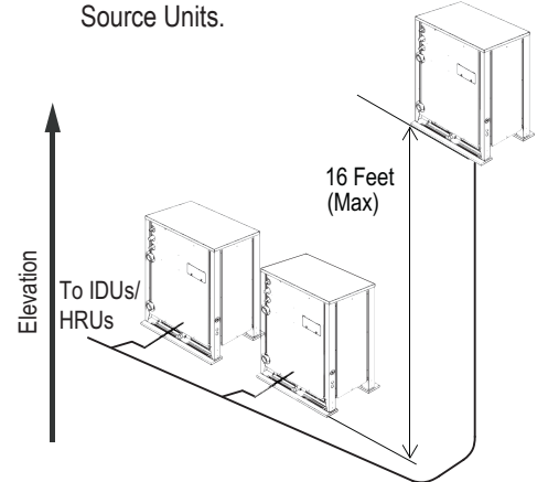
Figure 41: Traps for Heat Pump and Heat Recovery Units.
