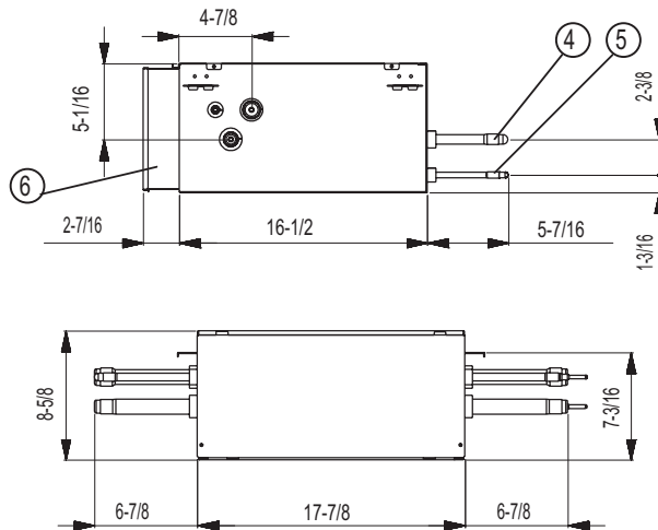
Figure 17: Heat Recovery Unit Dimensions.
