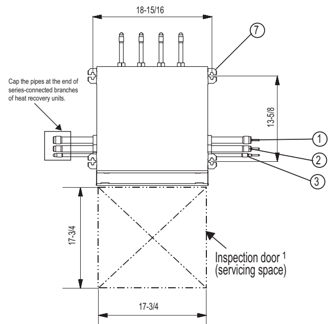
Figure 17: Heat Recovery Unit Dimensions.
