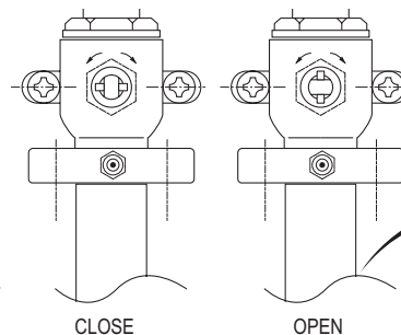
Figure 48: Service Valves - Open and Closed Positions.
