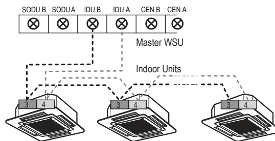
Communications Between IDUs and Master WSU
