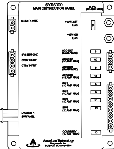
System 6000 Central Fuse Panel
