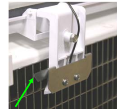
Ice Thickness Sensor Contact with water makes circuit from controller to cabinet, terminating freeze
