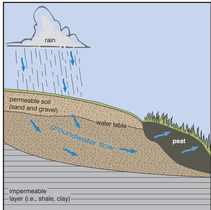
Generalized cross-section of an Iowa fen. Fens are groundwater fed wetlands. Determining the source and quality of recharge waters is important for their protection.
