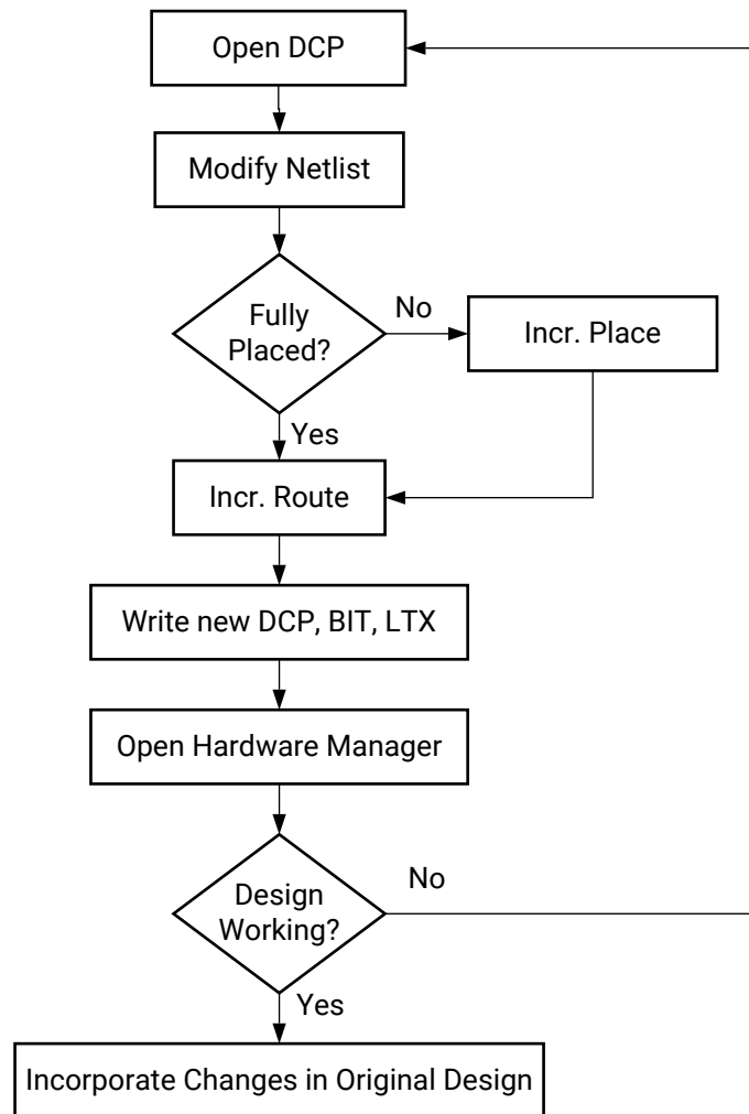
Figure 57: ECO Flow Chart
