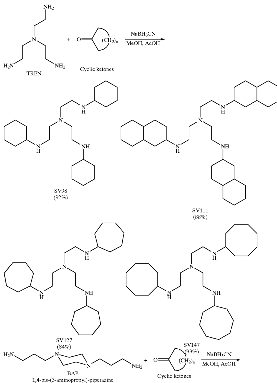
Scheme 1. Poly-(cycloalkyl-amines) obtained by reductive amination.
