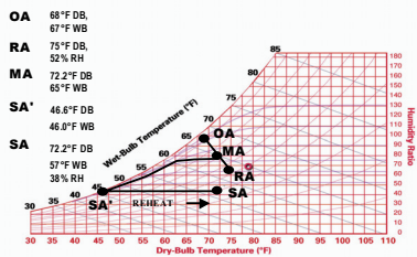
Figure 2. Psychrometric Chart
