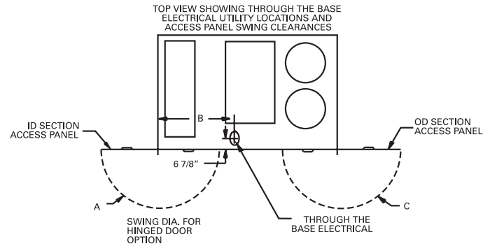
Figure 17. Cooling Unit - Swing Diameter & Through the Base Electrical
