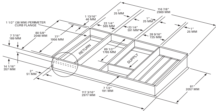
Figure 14. Cooling with Optional Electric Heat and Gas/Electric Models - 20-25 Tons Standard Efficiency; 15-25 Tons High Efficiency - Roof Curb
