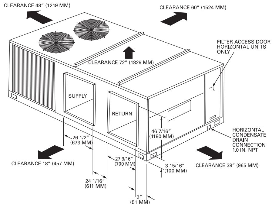
Figure 13. Cooling with Optional Electric Heat and Gas/Electric Models - 20-25 Tons Standard Efficiency; 15-25 Tons High Efficiency - Horizontal Unit Supply/Return and Unit Clearance
