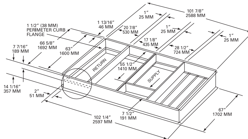
Figure 9. Cooling with Optional Electric Heat and Gas/Electric Models 12½-17½ Tons Standard Efficiency - 12½ Tons High Efficiency - Roof Curb
