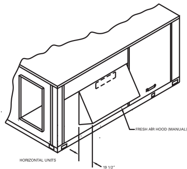
Figure 19. Fresh Air Hood (Horizontal Units)
