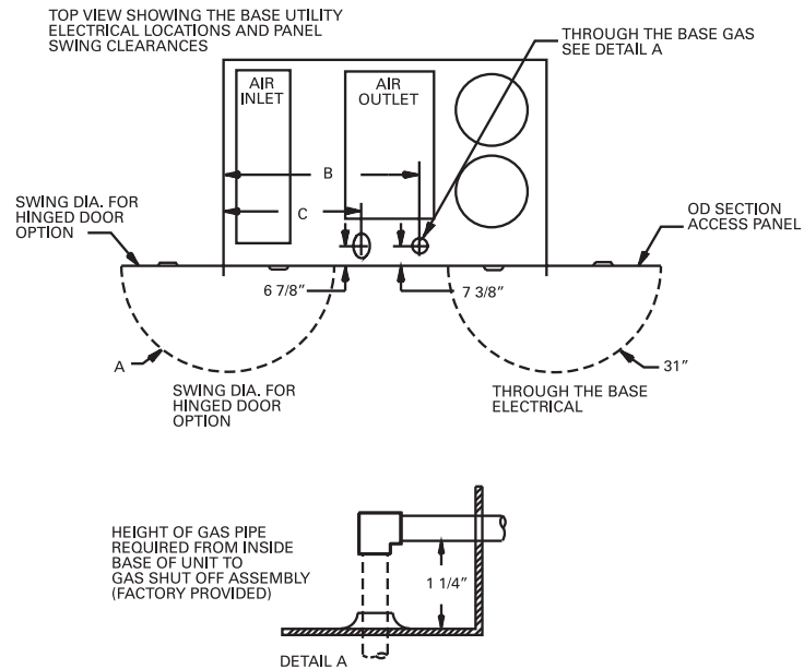
Figure 18. Gas/Electric Unit - Swing Diameter & Through the Base Electrical; Height of Gas Pipe (Second Drawing)
