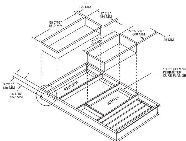
Figure 10. Cooling with Optional Electric Heat and Gas/Electric Models 12½-17½ Tons Standard Efficiency; 12½ High Efficiency - Downflow Duct Connections - Field Fabricated
