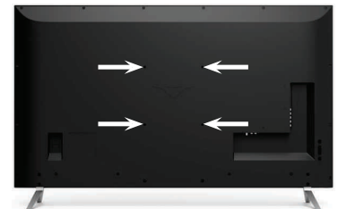
WALL-MOUNT SCREW LOCATIONS
