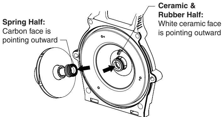
Mechanical Seal
