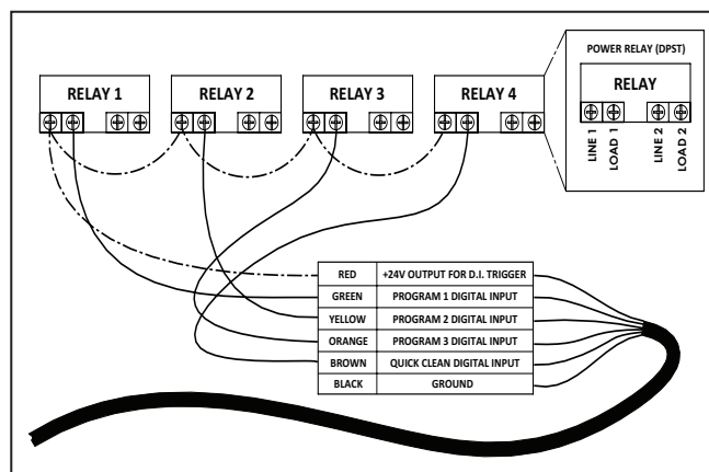
Figure 12: External Control Wiring Diagram
