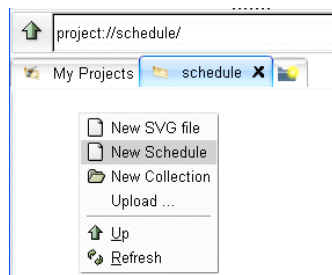
FIG. 35 Schedule menu
