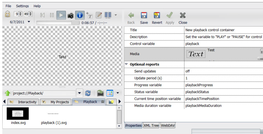
FIG. 90 Playback.svg details
