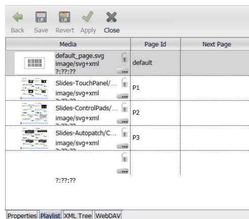
FIG. 43 Playlist
