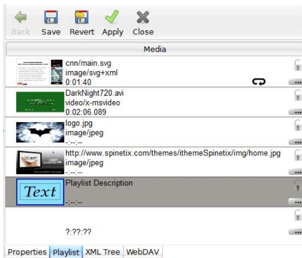
FIG. 18 Playlist Tab
