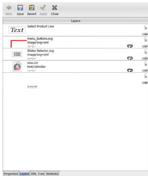
FIG. 117 Layers pane
