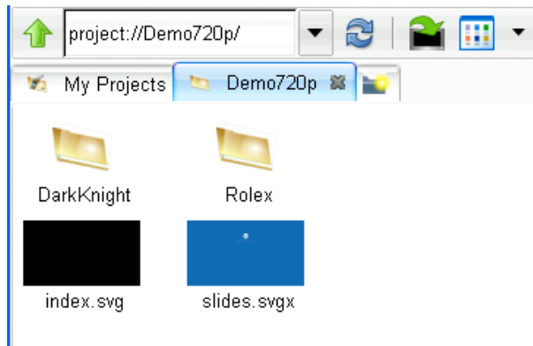
FIG. 27 Demo720p Folder
