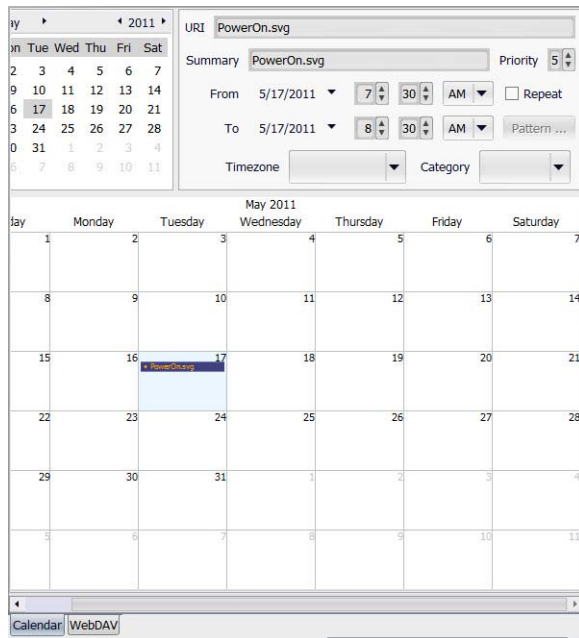
FIG. 116 new.ics file
