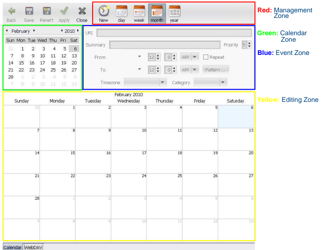
FIG. 36 Calendar view
