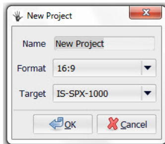
FIG. 86 New Project
