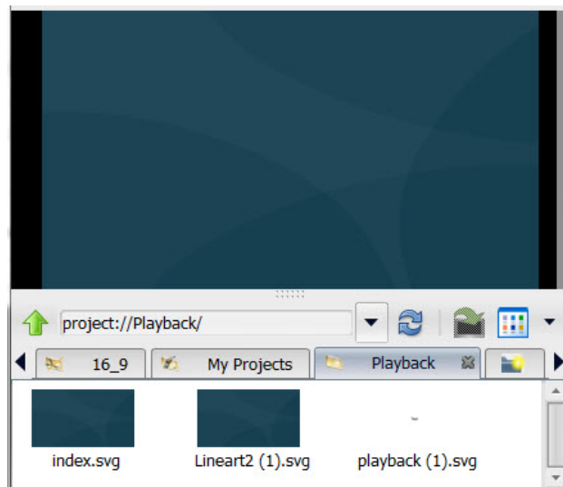
FIG. 91 Added background
