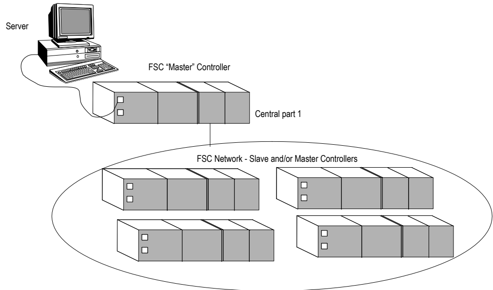
Figure 1-5: FSC network
